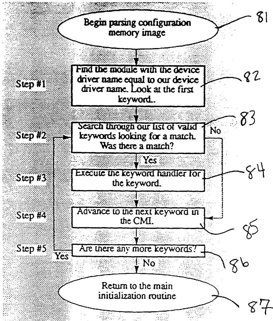
Configuration Memory Image Parsing Flow Chart
