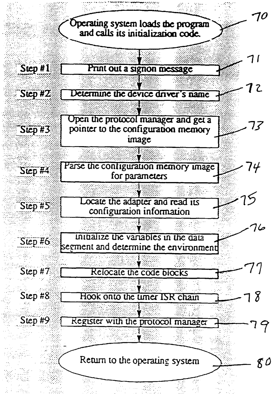
Initialization Process Flow Chart
