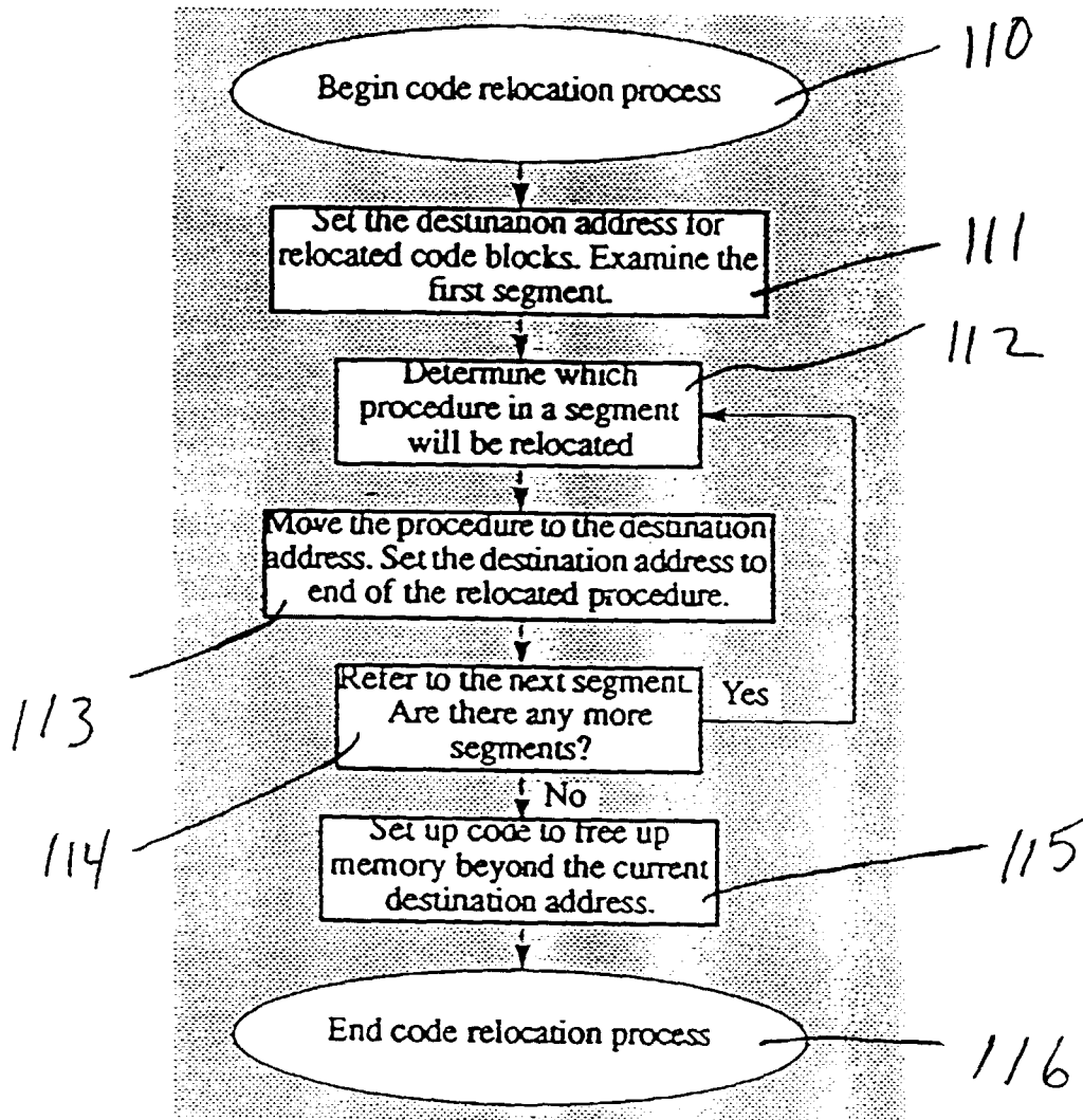
Code Relocation Flow Chart
