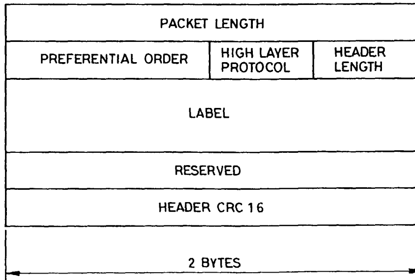
HEADER STRUCTURE IN CASE OF IPv4 AND IPv6 FOR TRANSFERRING USING LABEL TECHNOLOGY
