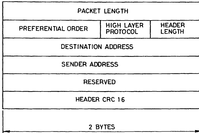
HEADER STRUCTURE IN CASE OF ATM
