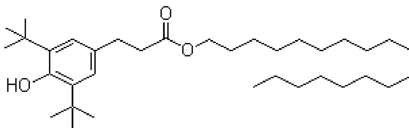
Phenolic Primary Antioxidant: Irganox 1076
