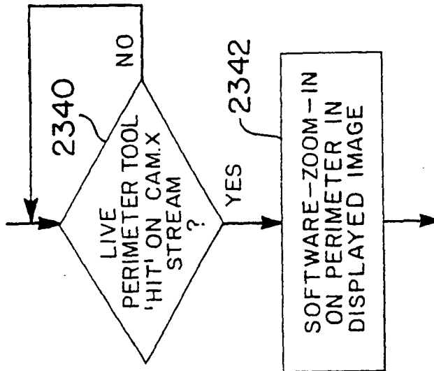
FIG. 108 SOFT-ALARM-ACTUATED ZOOM-IN
