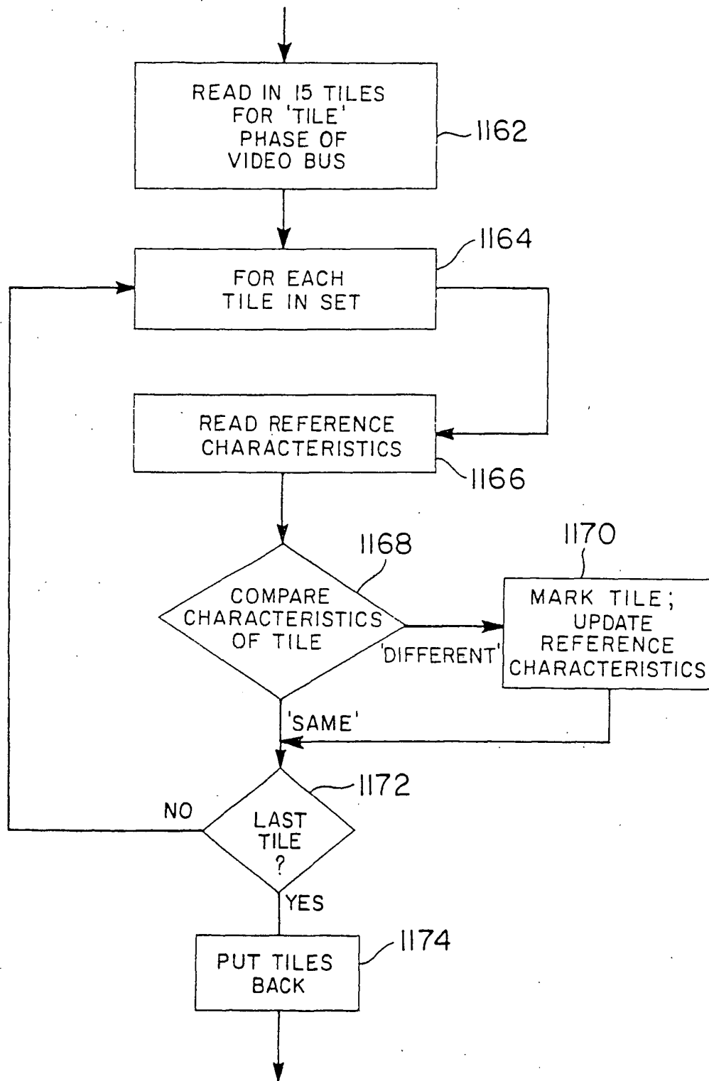
FIG. 42 TILE COMPARING
