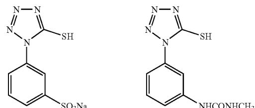
Mercapto compound-1
