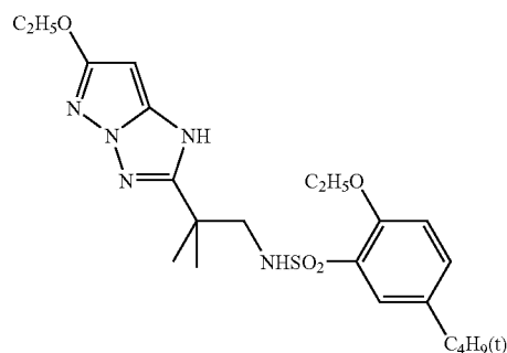
(3-20)
