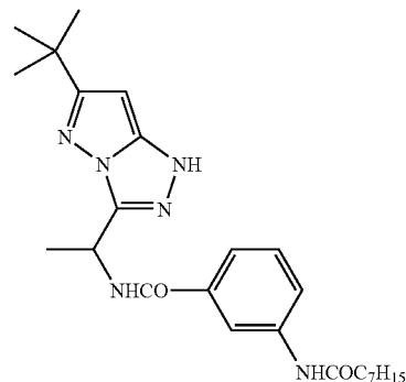
(4-3)
