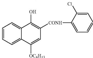
Development accelerator-2
