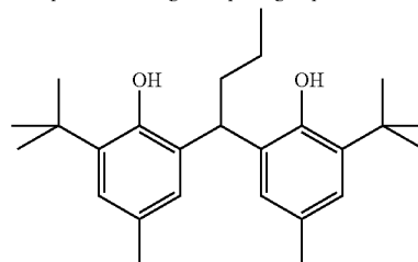
Reducing agent-1
