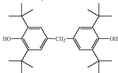
Color-tone-adjusting agent-1
