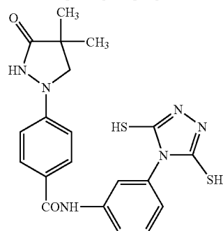
Compound 2 having adsorptive group and reducing group
