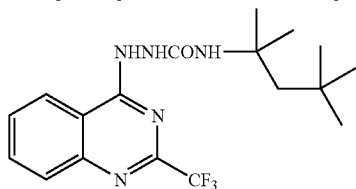
Development accelerator-1
