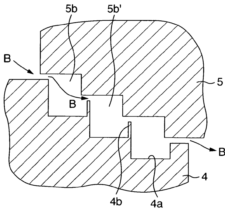
FIG.6 PRIOR ART
