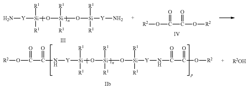
Reaction Scheme A
