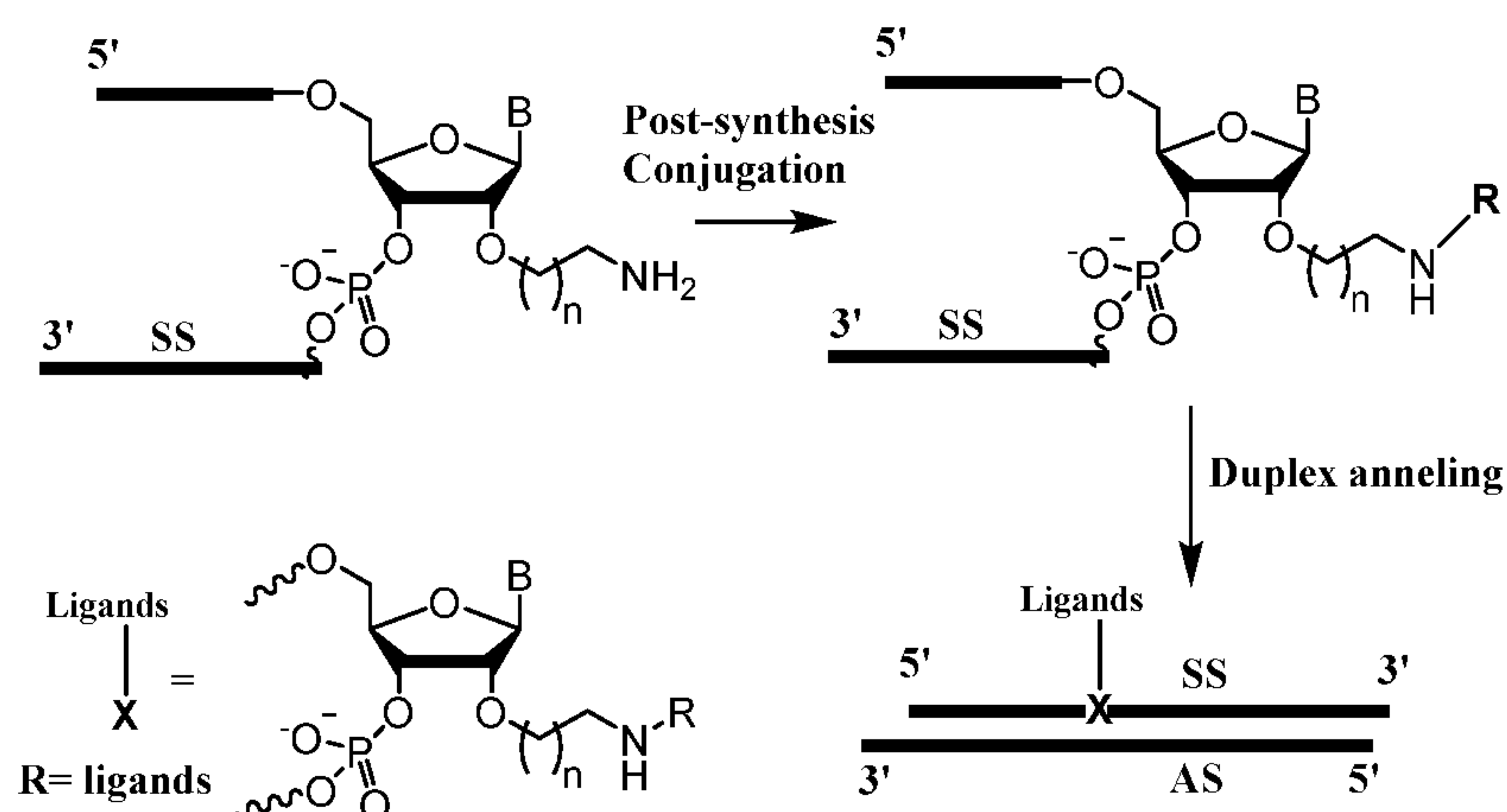
Scheme 61
