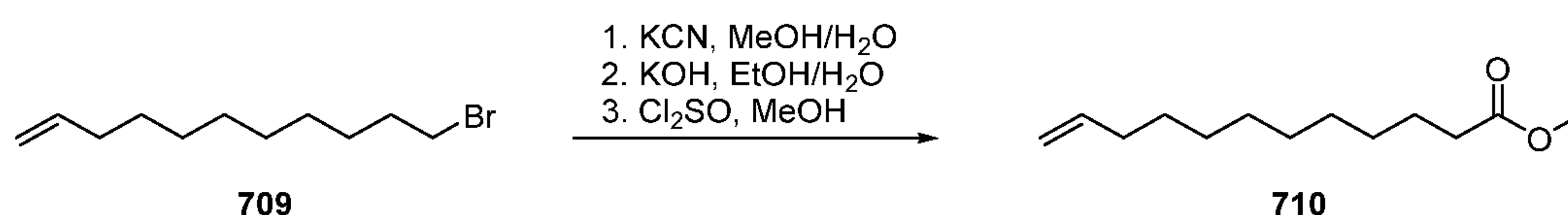
Scheme 34
