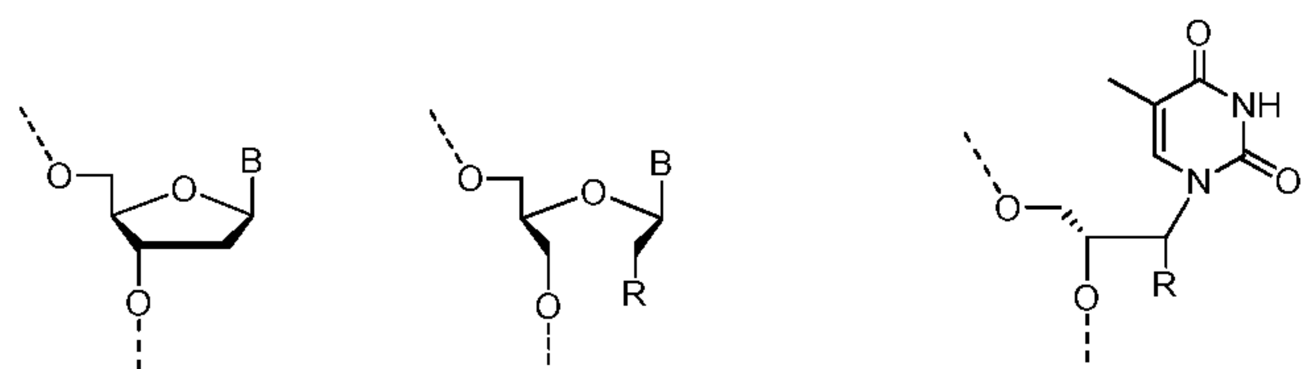
unlocked nucleic acid R= H, OH, O-alkyl
