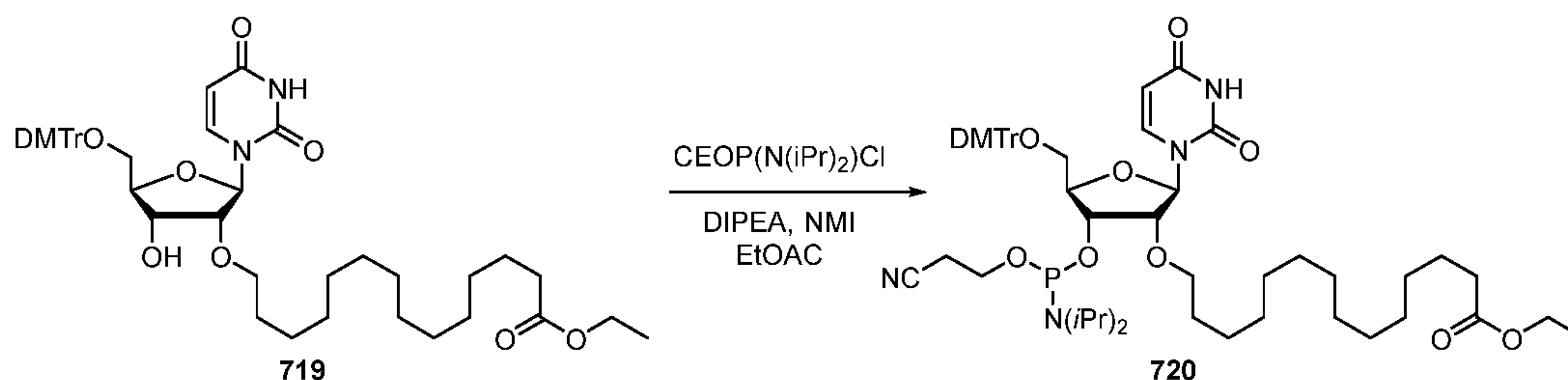
Scheme 44
