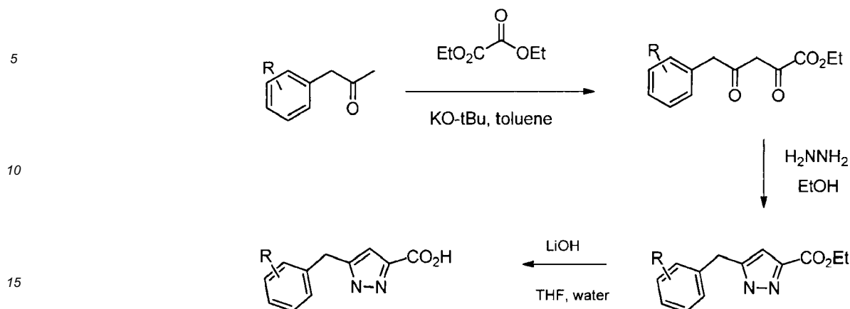
Scheme 7
