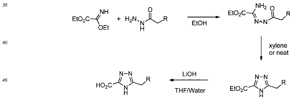
Scheme 6
