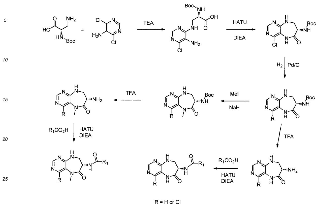
Scheme 4
