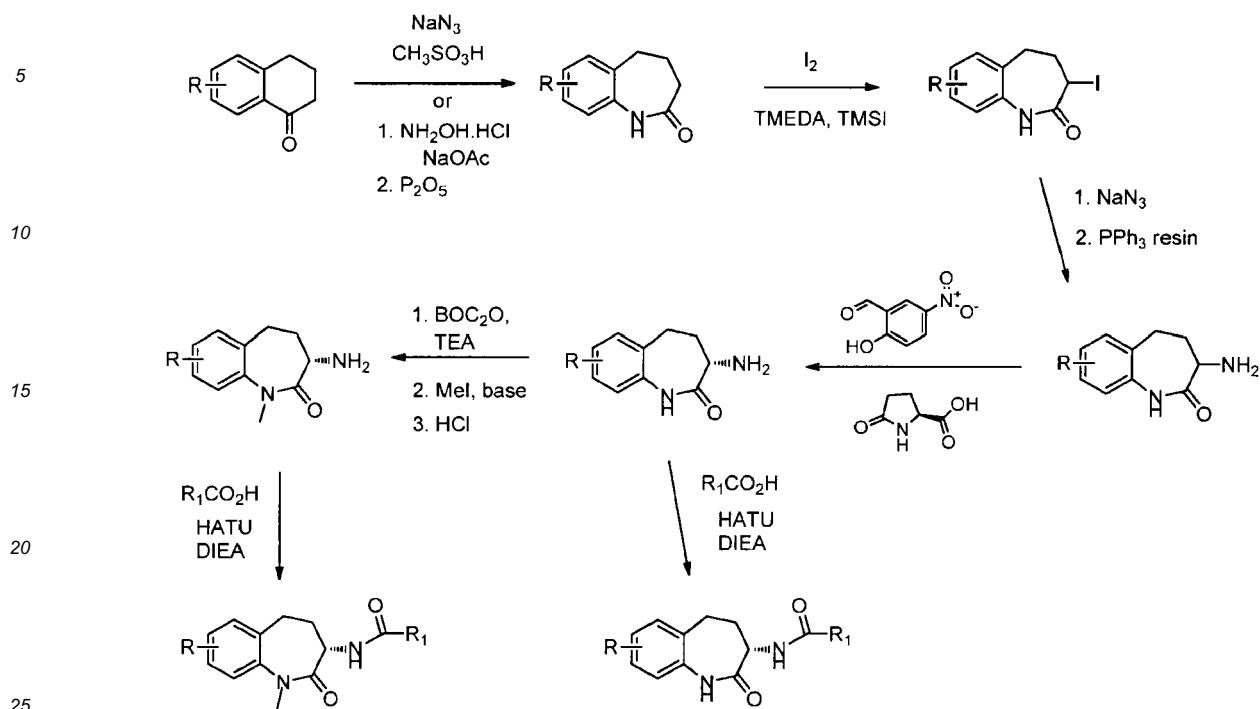
Scheme 5
