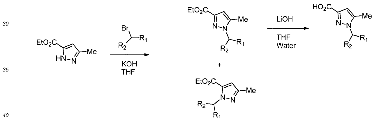
Scheme 8
