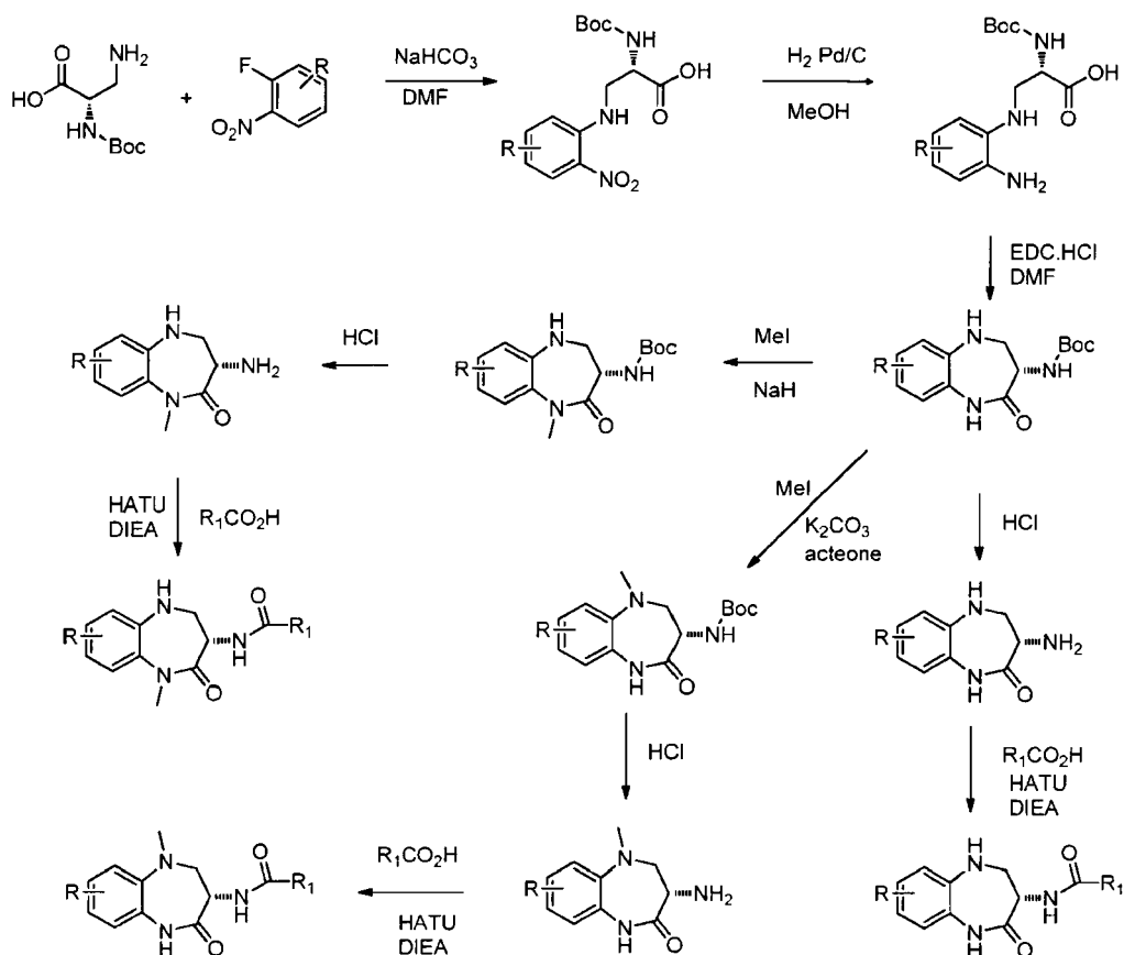
Scheme 3
