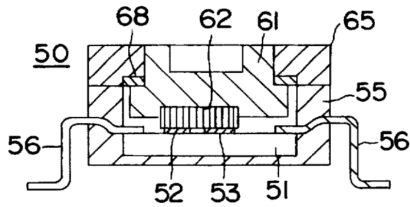
FIG. 12 PRIOR ART
