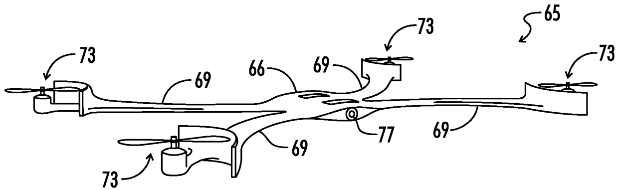
FIG. 3 (PRIOR ART)
