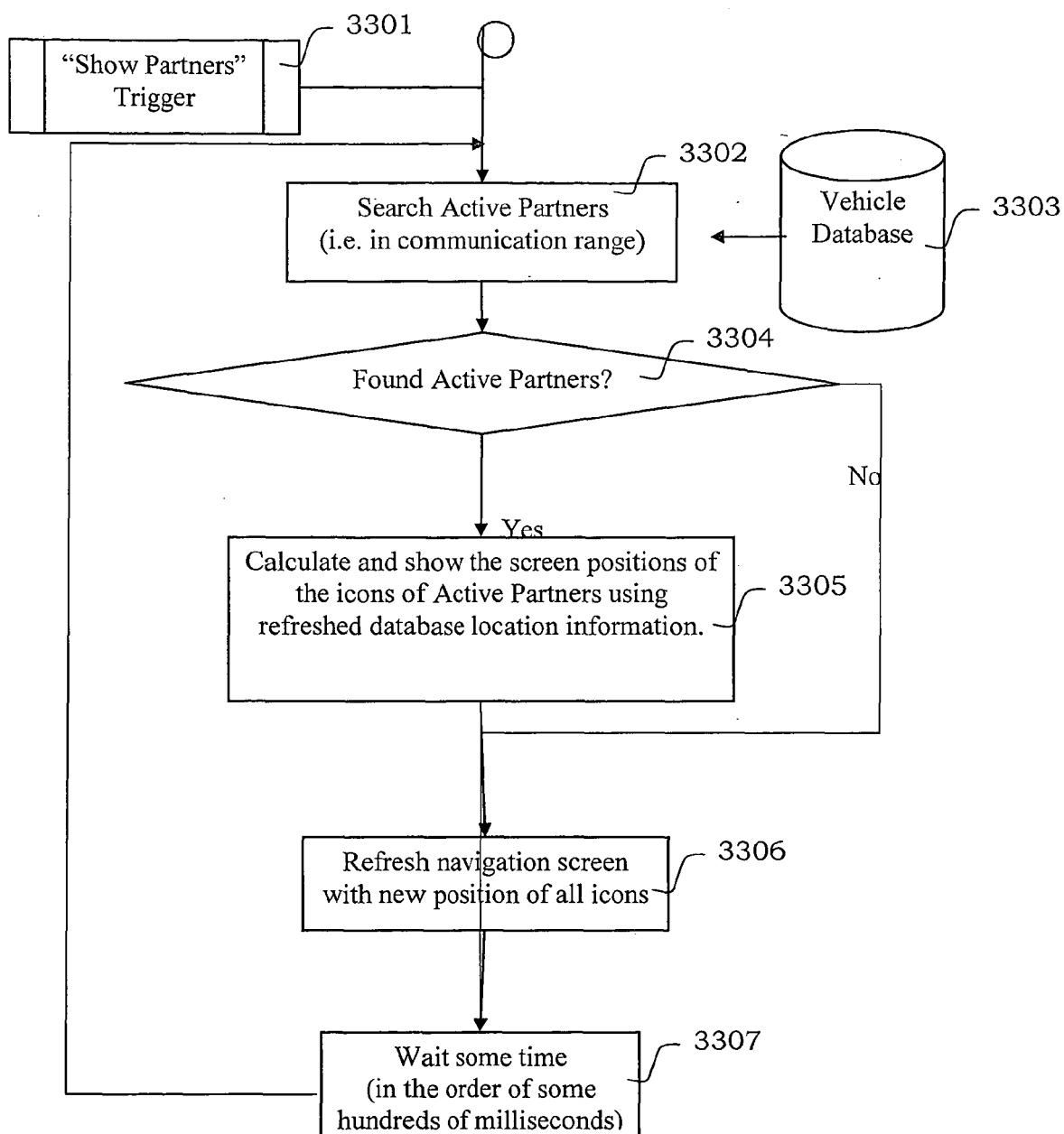
Figure 33: Flow Chart for Displaying Partners
