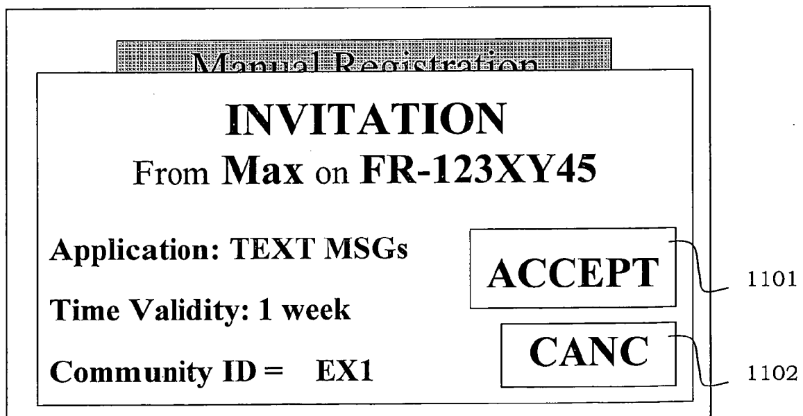
Figure 11: Invitation screen
