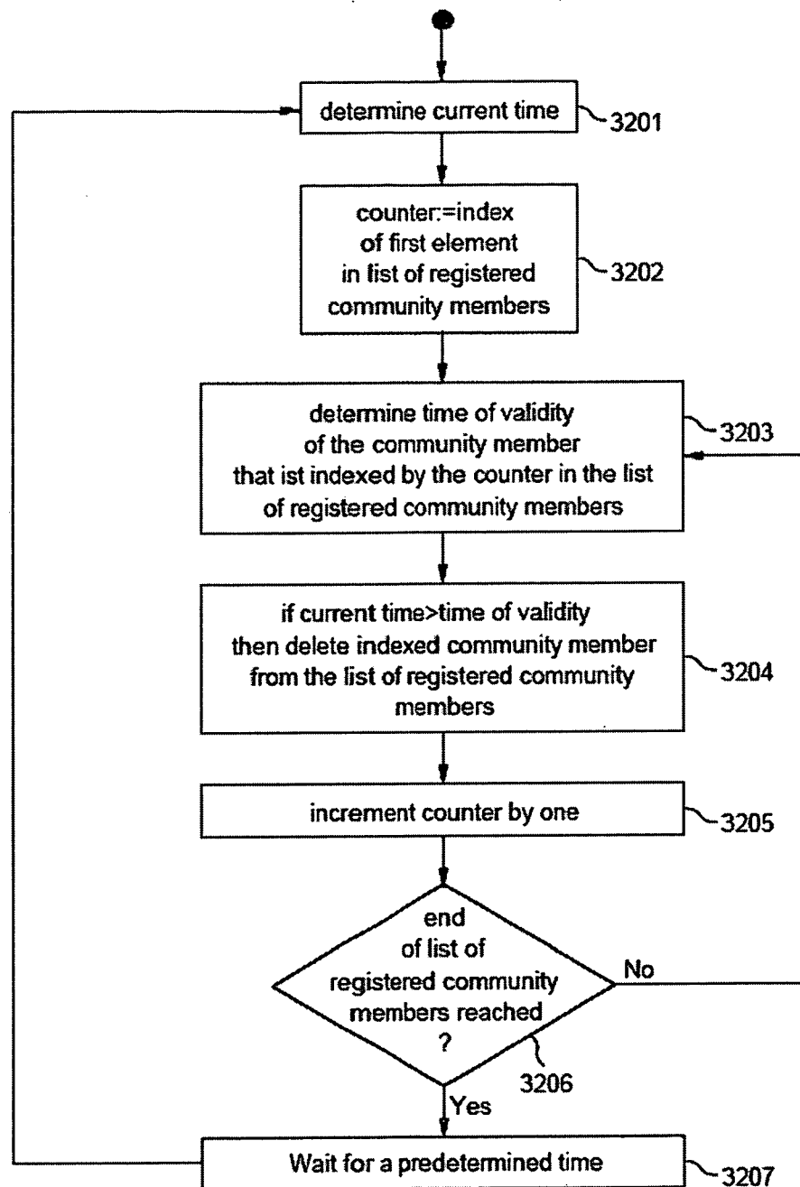
Figure 32: Garbage collection
