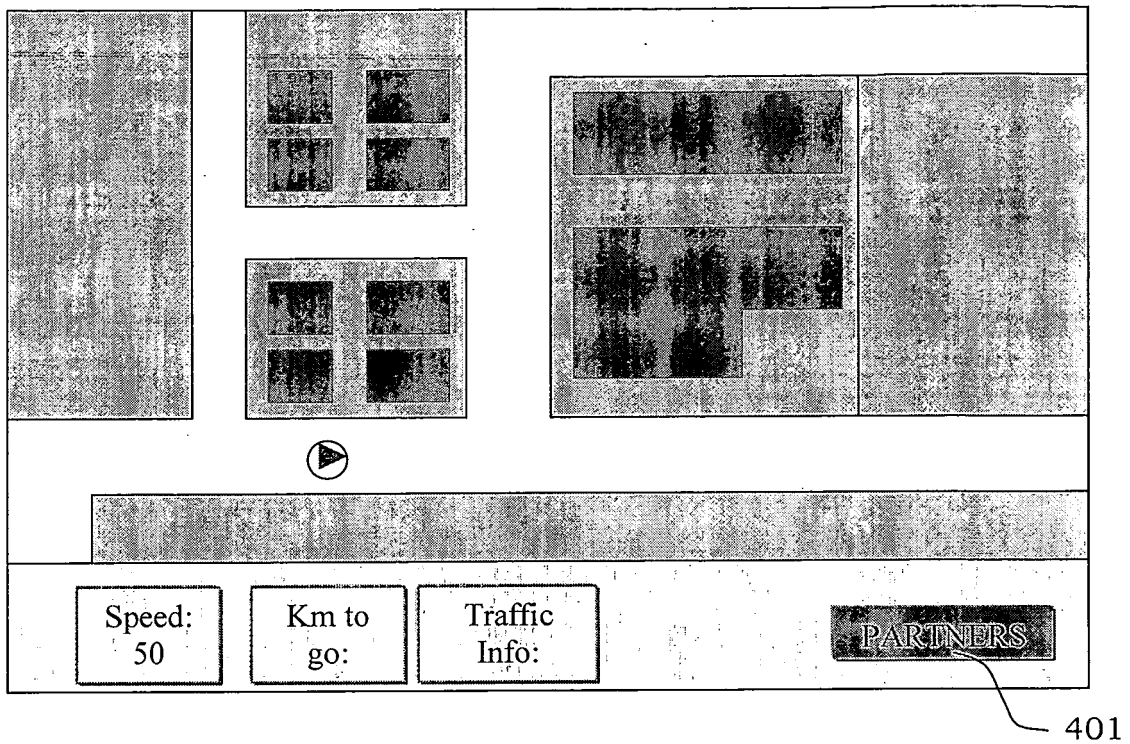
Figure 4: Navigation screen
