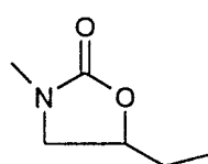
(A) (Racemat)
