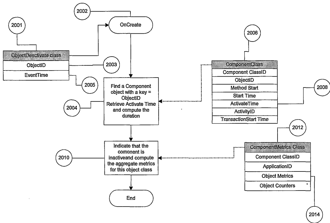
Figure 20: Algorithm for Handling Object Deactivation
