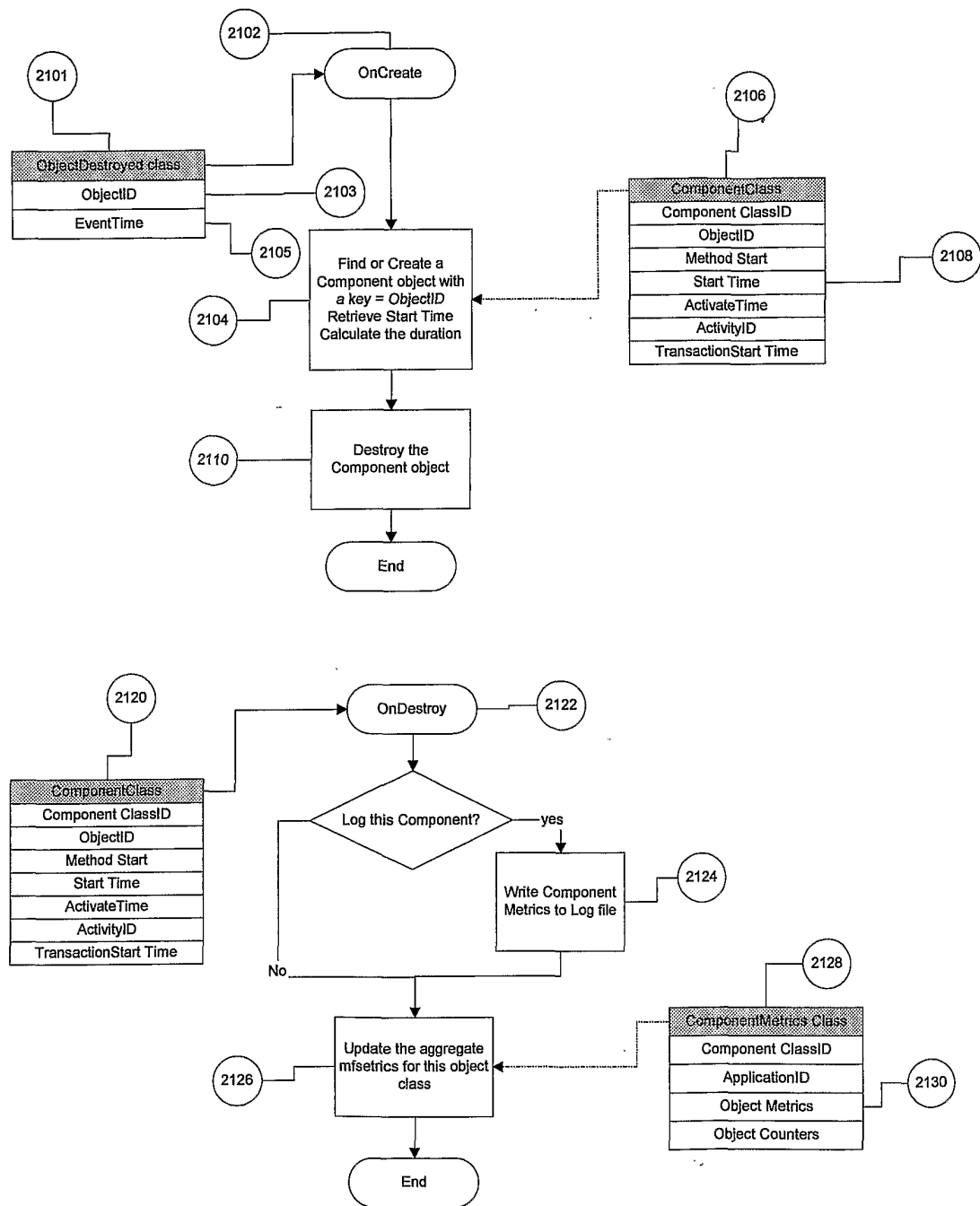
Figure 21: Algorithm for Handling Object Destruction
