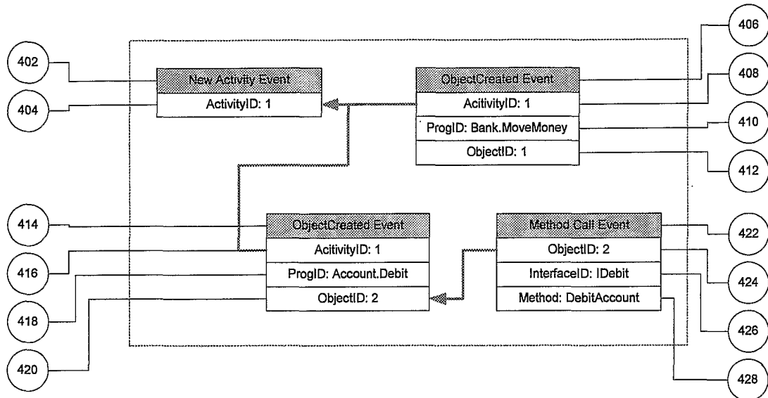
Figure 4: Correlation of Transaction Object Events
