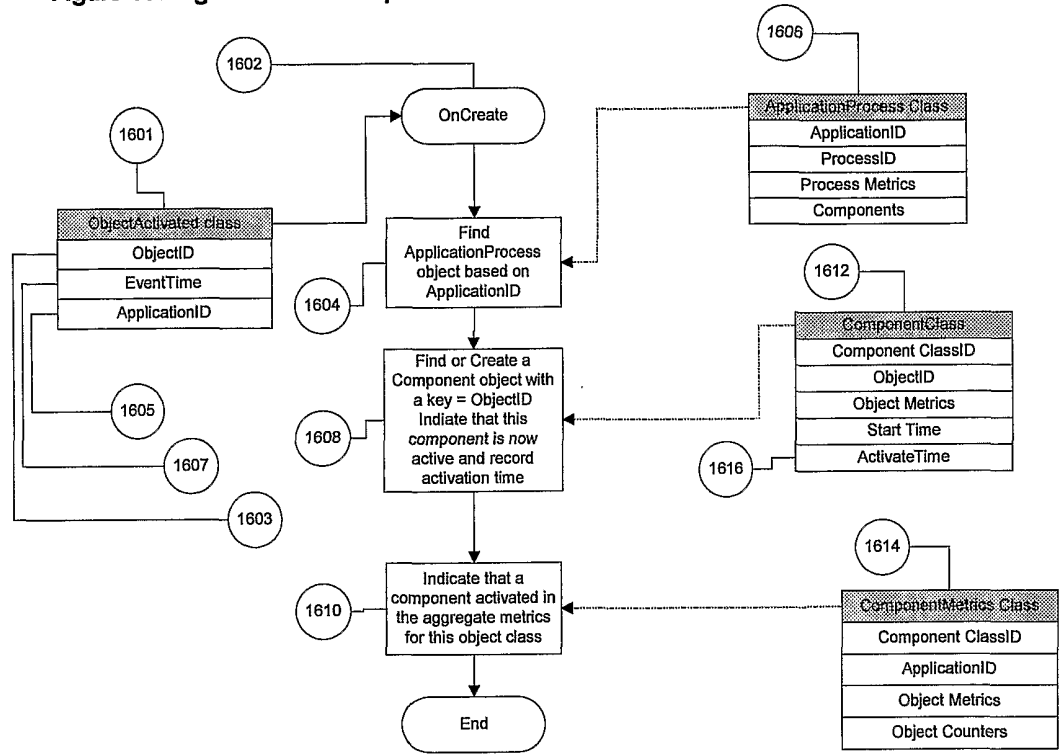
Figure 16: Algorithm for Component Activation
