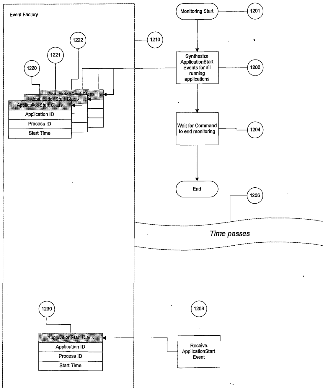
Figure 12: Algorithm for Application and Process Metrics - Application Startup
