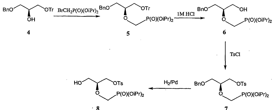
Scheme 3: Synthesis of (S)-1-[hydroxy-2-(phosphonomethoxy)propyl]-5-azacytosine from the HPMP-synthon
