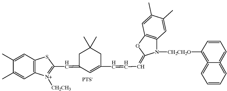
Sensitizing dye A
