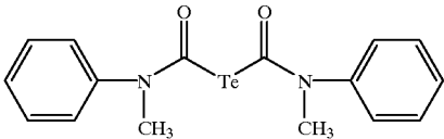
Base precursor compound 11
