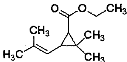
Ethyl Chrysanthemumate
