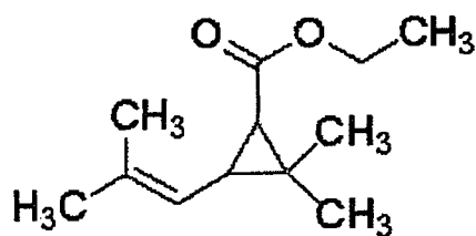
Ethyl Chrysanthemumate
