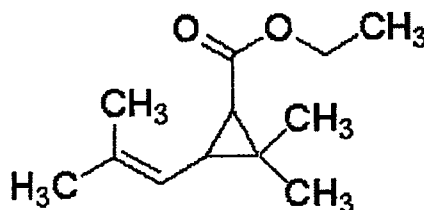
Ethyl Chrysanthemumate
