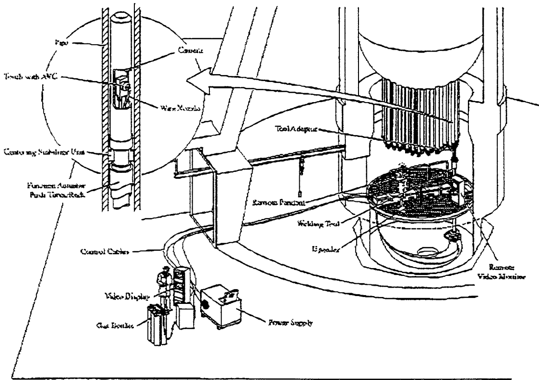
Welding System with Weld Head Installed
