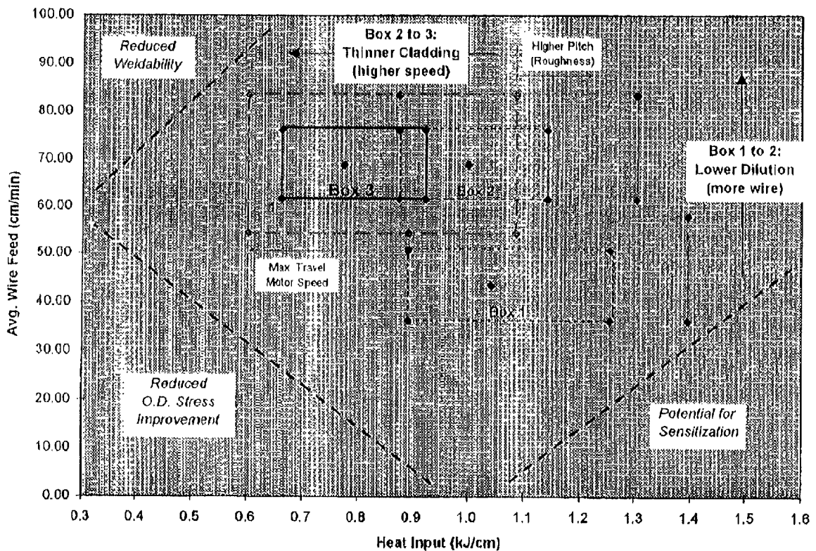
Heat Boxes 1, 2, 3 (with Reference Points)
