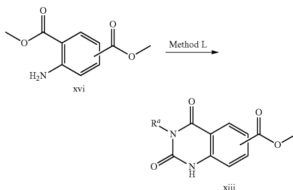
Scheme 6: General route for the preparation of 3-substituted 2,4-dioxo-1,2,3,4-tetrahydroquinazoline 6-, or 7-carboxylates
