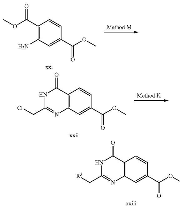
Scheme 9: General route for the preparation of substituted 4-oxo-3,4-dihydroquinazoline-7-carboxylates
