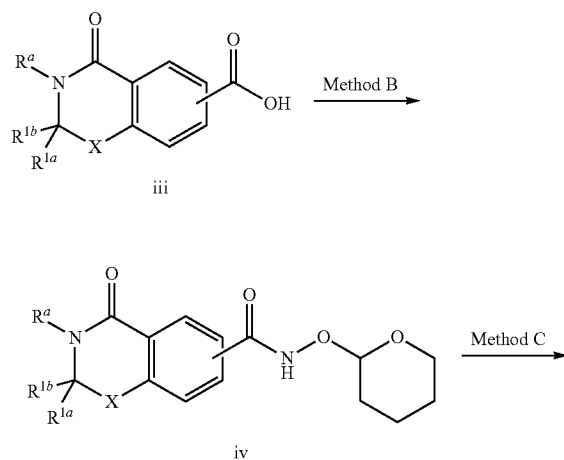
Scheme 2: General route 2 for the preparation of hydroxamates
