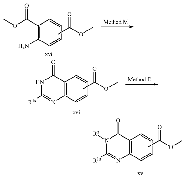
Scheme 7: General route for the preparation of di-substituted 4-oxo-3,4-dihydroquinazoline 6-, or 7-carboxylates
