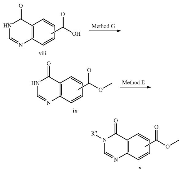
Scheme 4: General route for the preparation of 3-alkyl methyl 4-oxo-3,4-dihydroquinazoline 6-, or 7-carboxylates
