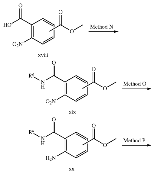
Scheme 8: General route for the preparation of di-substituted 4-oxo-3,4-dihydroquinazoline 6-, or 7-carboxylates
