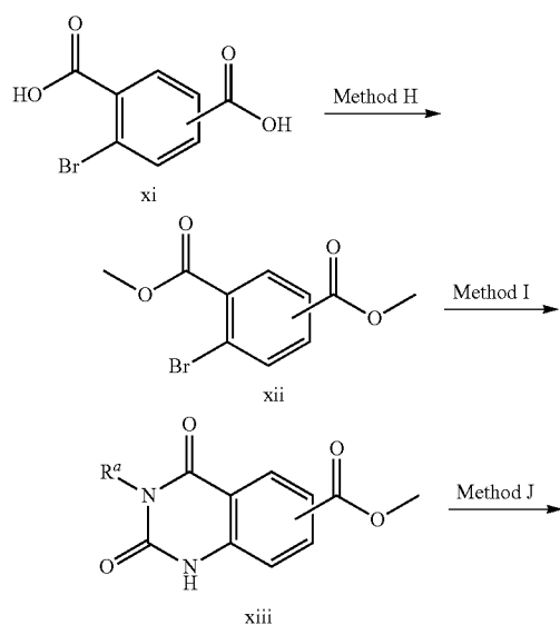
Scheme 5: General route for the preparation of di-substituted 4-oxo-3,4-dihydroquinazoline 6-, or 7-carboxylates
