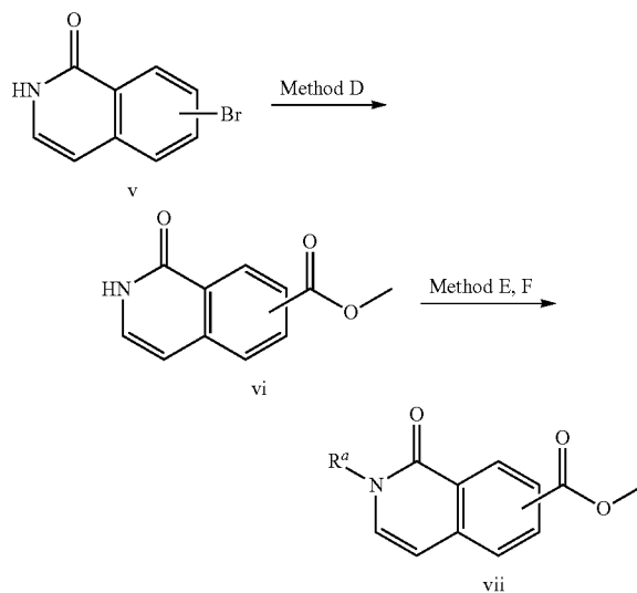
Scheme 3: General route for the preparation of 2-alkyl or aryl methyl 1-oxo-1,2-dihydroisoquinoline 6-, or 7-carboxylates
