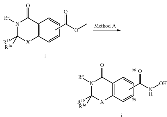
Scheme 1: General route 1 for the preparation of hydroxamates
