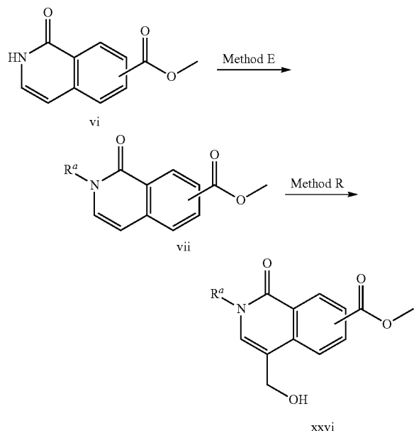
Scheme 11: General route for the preparation of 4-(hydroxymethyl) substituted 2-alkyl methyl 1-oxo-1,2-dihydroisoquinoline 6-, or 7-carboxylates
