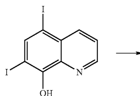
Scheme 10
