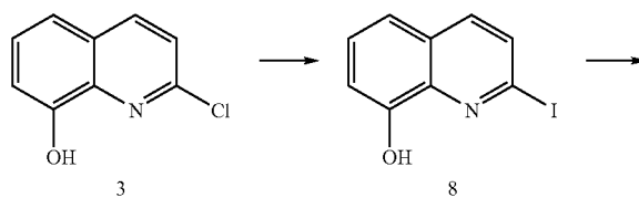
Scheme 12
