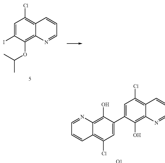
Scheme 11
