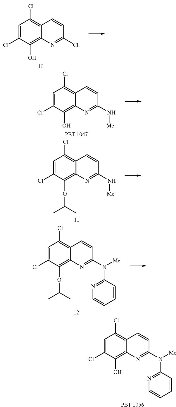
Scheme 13
