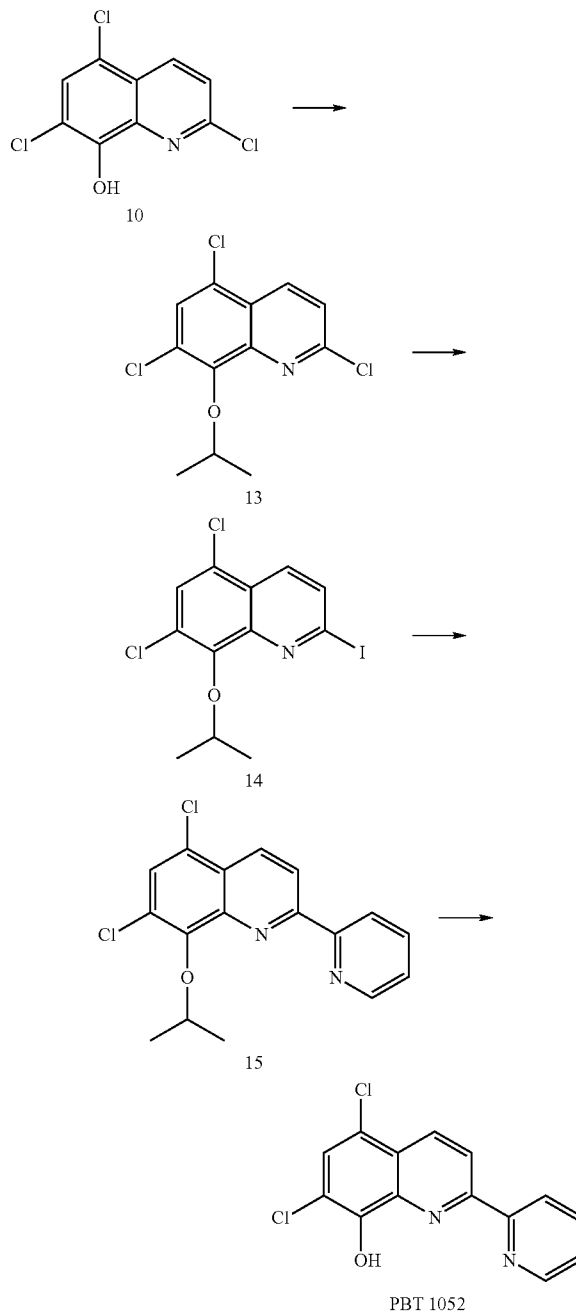
Scheme 14
