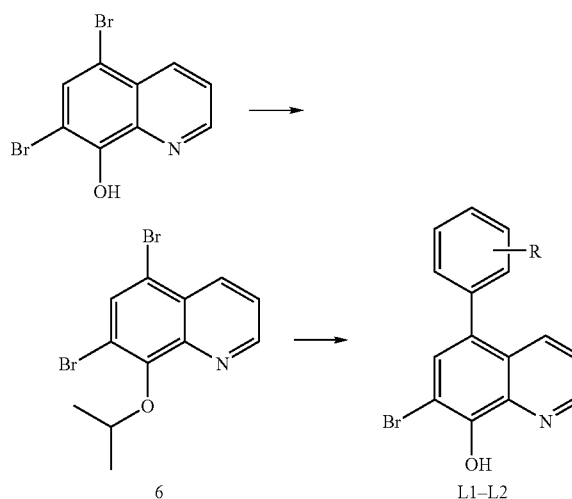
Scheme 9
