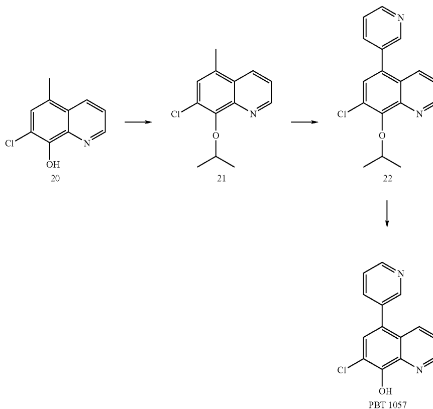
Scheme 17
