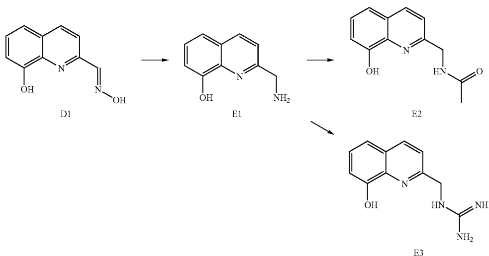
Scheme 4
