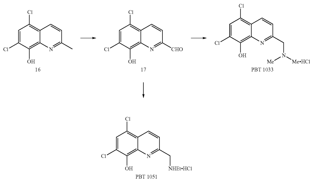
Scheme 15
