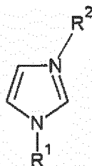
(Chemical Formula 2)
