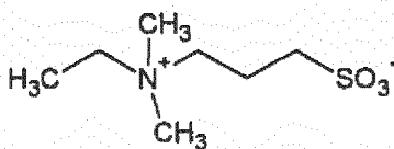
(Chemical Formula 5)
