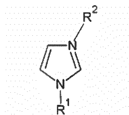
(Chemical Formula 2)
