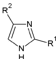
(Chemical Formula 2)
