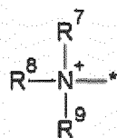
(Chemical Formula 3-4)
