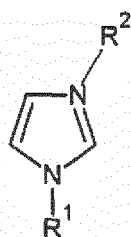
(Chemical Formula 2)
