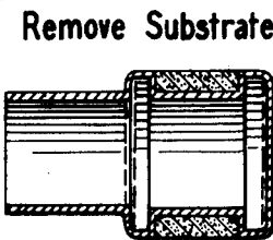
Fig. 4. Cut Out Cavity Section
