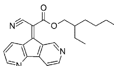
Compound 6
