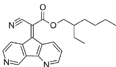
Compound 3
