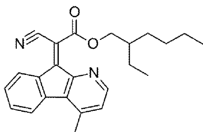
Compound 7
