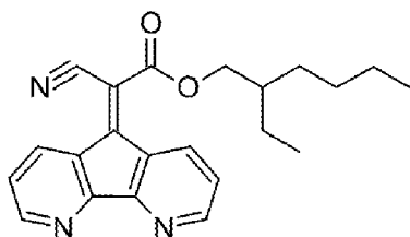
Compound 5
