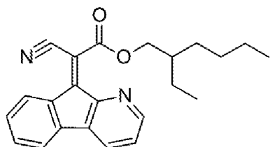
Compound 1
