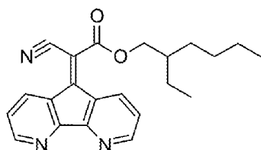
Compound 5
