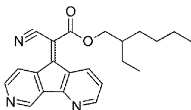
Compound 3
