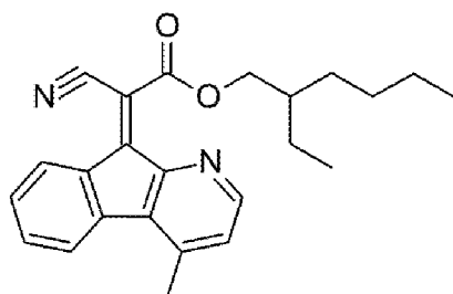
Compound 7
