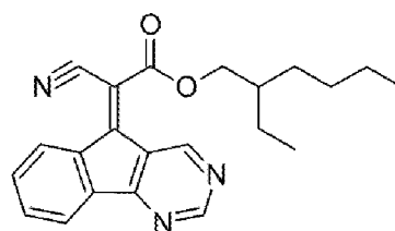
Compound 2
