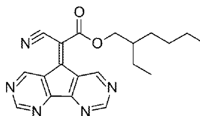
Compound 4
