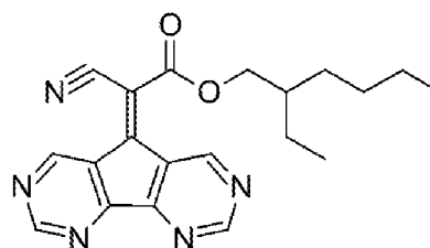
Compound 4
