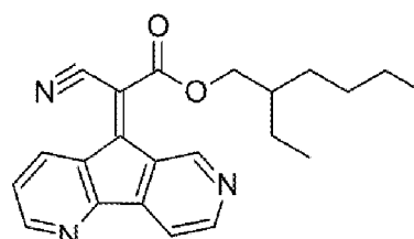
Compound 6
