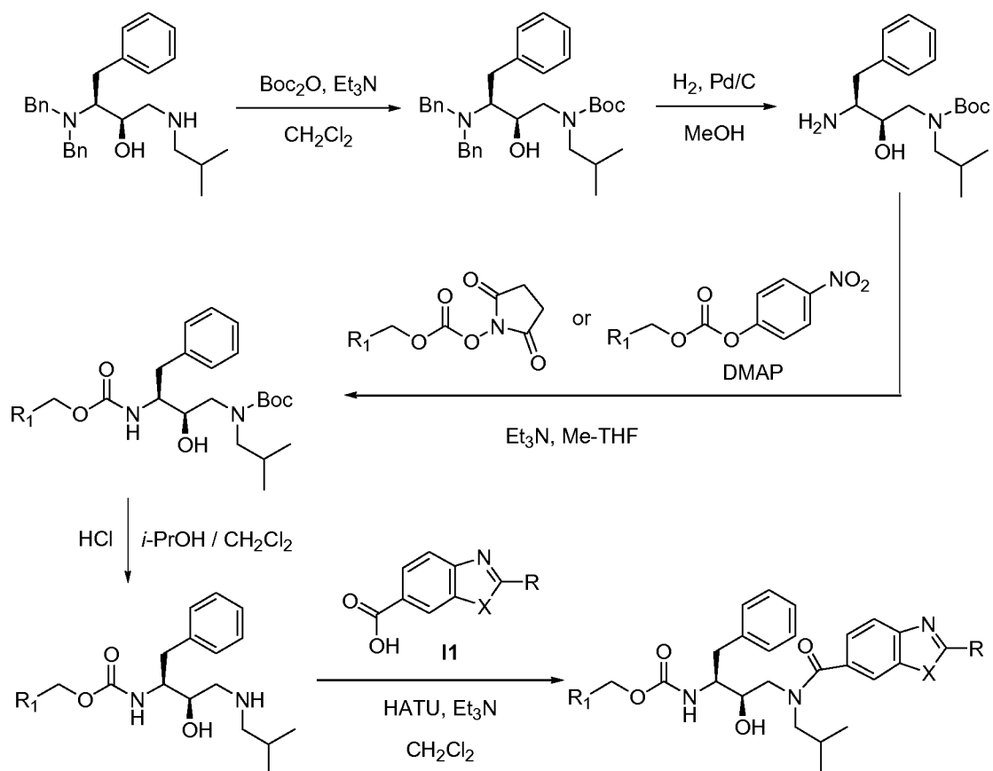
Scheme 3: Method 3
