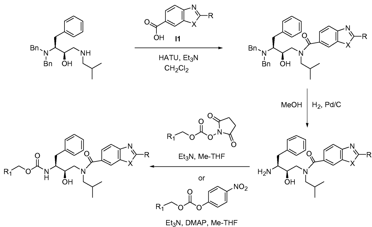
Scheme 2: Method 2
