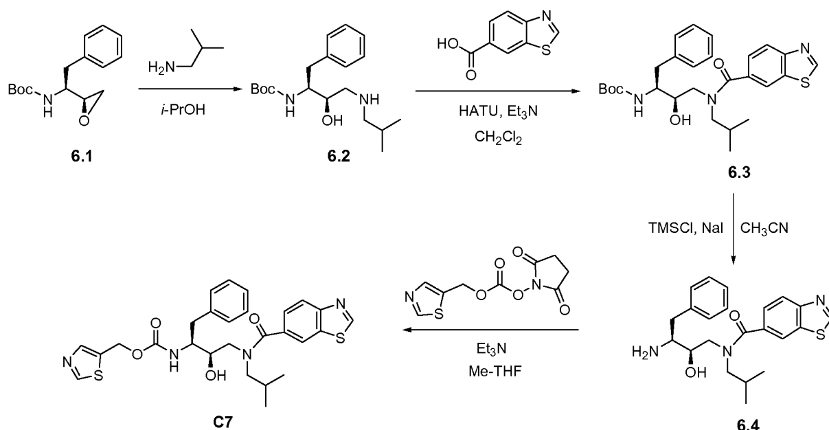
Scheme 6: Synthesis of thiazol-5-ylmethyl (2S,3R)-3-hydroxy-4-(N-isobutylbenzo[d]thiazole-6-carboxamido)-1-phenylbutan-2-ylcarbamate (C7)
