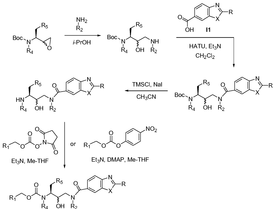
Scheme 1: Method 1
