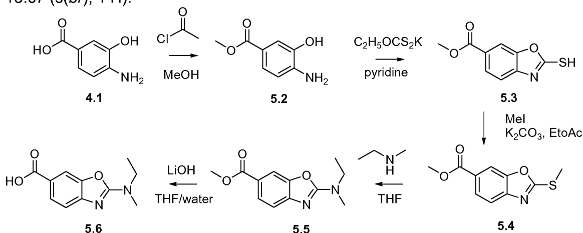
Scheme 5: Synthesis of 2-(ethyl(methyl)amino)benzo[d]oxazole-6-carboxylic acid (5.6)
