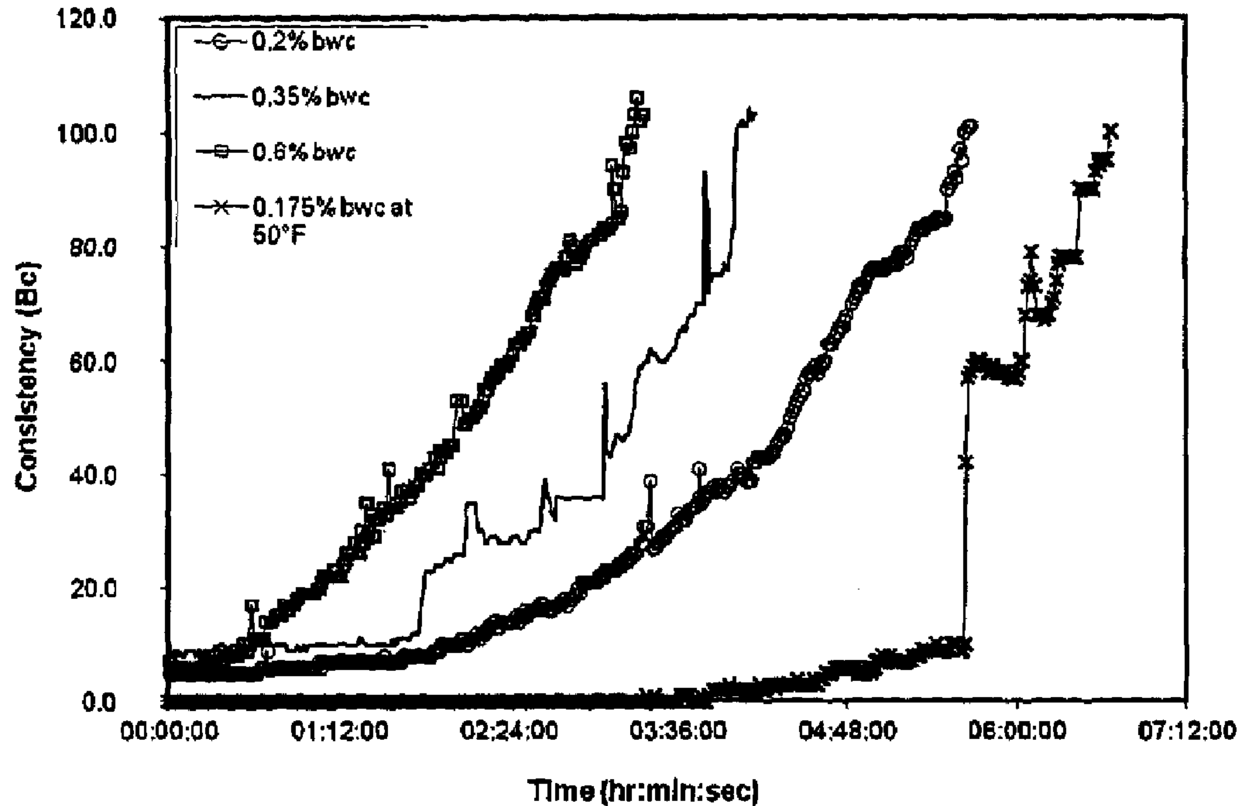
Graph of Consistency versus Time for varying concentrations of C-S-H seeds
