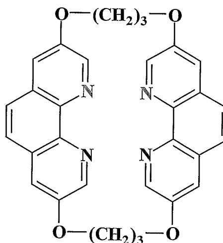
molecule G = Cyclo-bi-Phen
