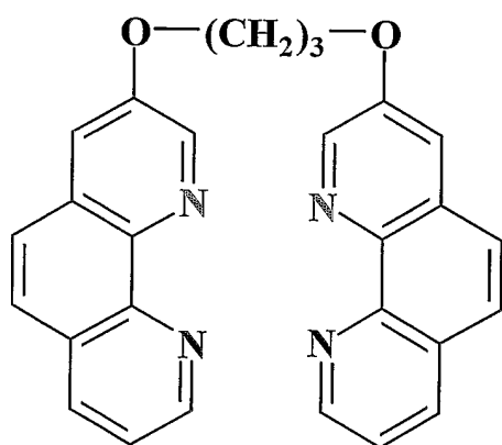
molecule B = 3-propyl-Clip-Phen (Phen = ortho-phenanthroline)
