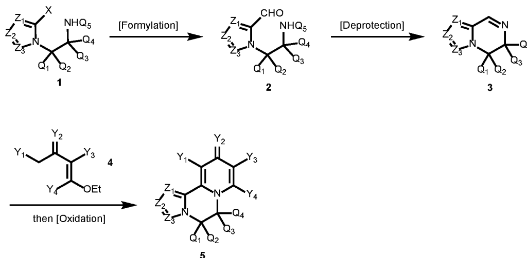
Scheme 32:
