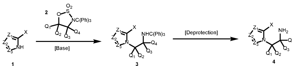
Scheme 36:
