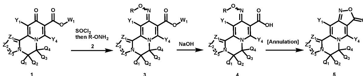
Scheme 30:
