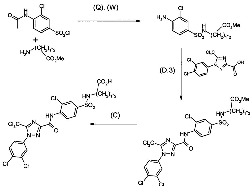
Scheme XII: General synthetic route to triazole amides (general procedures Q, W, D.3, C)
