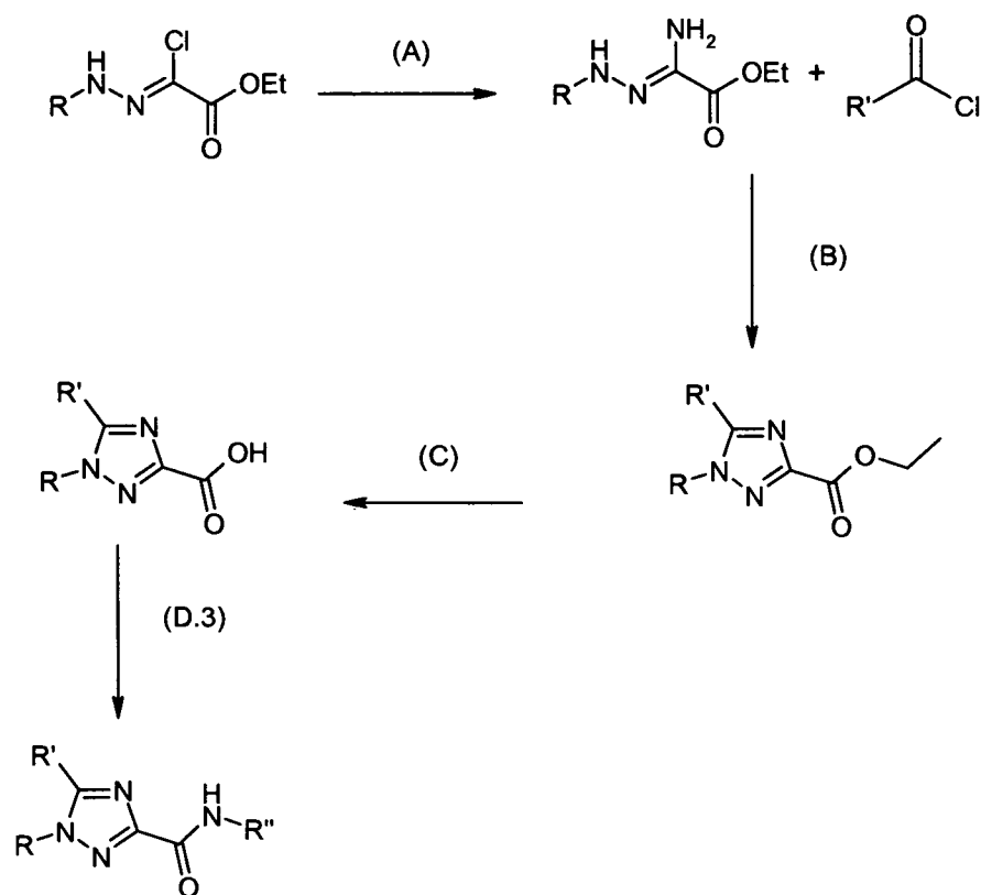
Scheme I: General route to 1H-[1,2,4]triazole-3-carboxamides (general procedures A, B, C, D.3)
