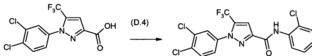
Scheme XIII: General synthetic route to pyrazole amides (general procedure D.4)
