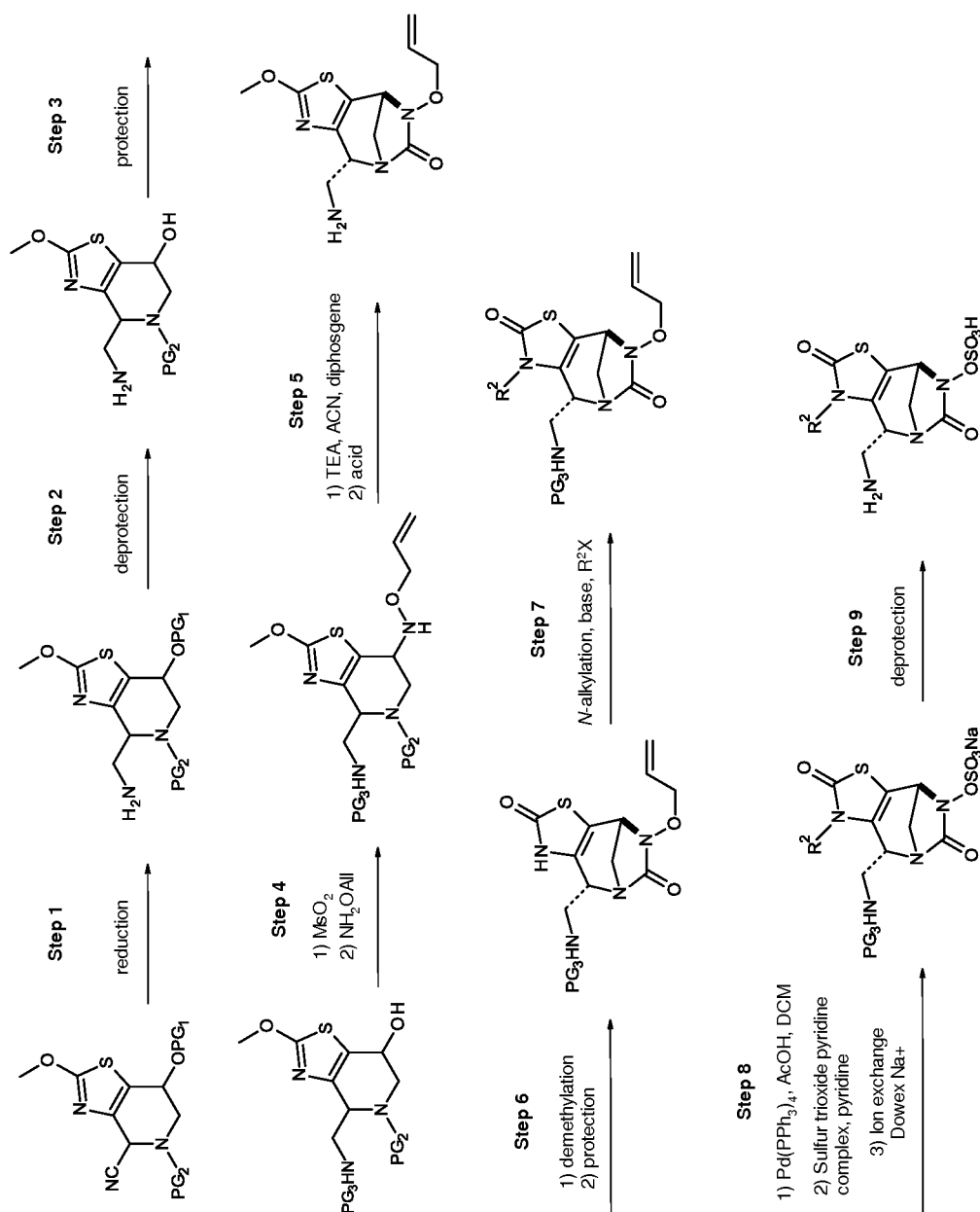
Scheme 6
