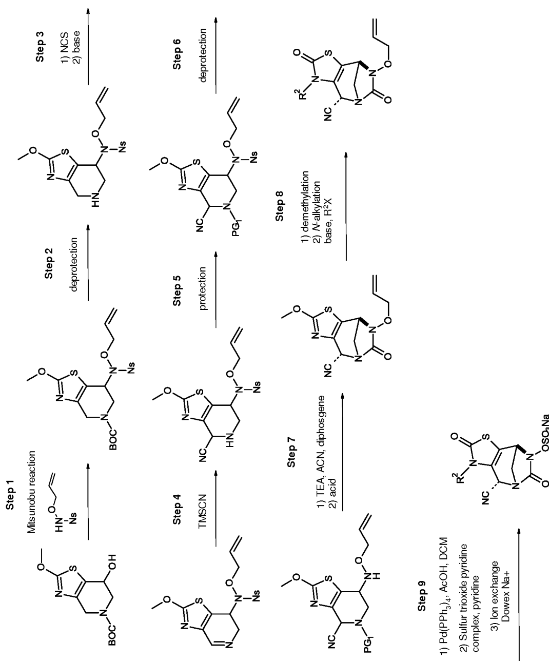
Scheme 5
