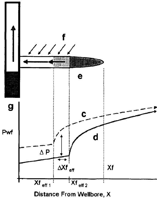
Figure 1B: Well After Process
