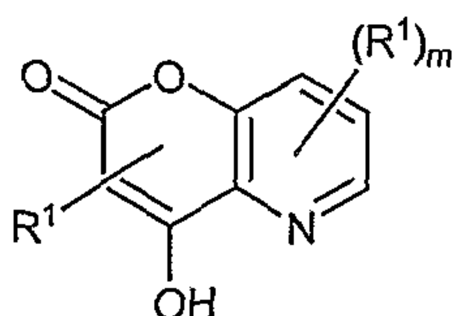
4-hydroxy-4a,8a-dihydro-pyrano[3,2,b]pyridin-2-one
