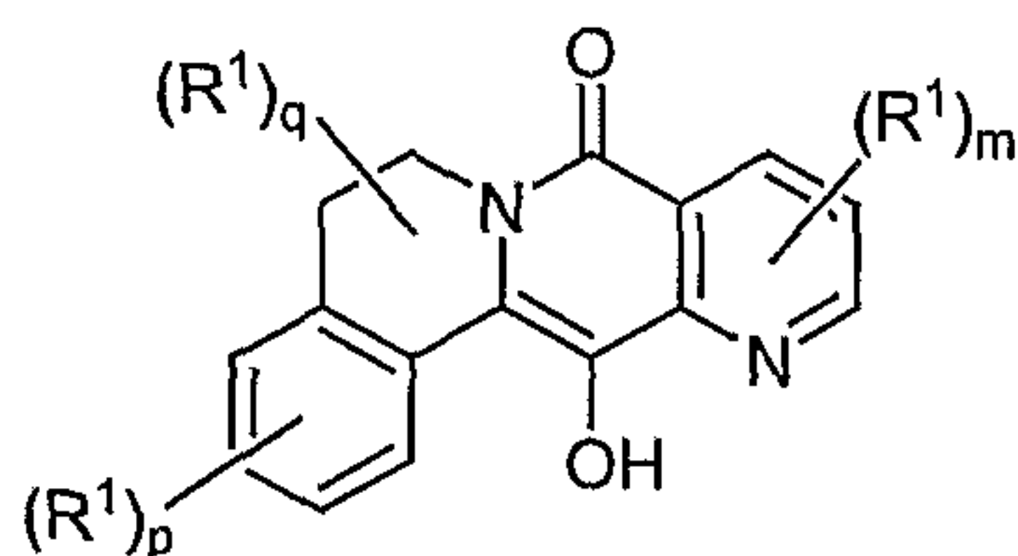
dibenzo[a,g]quinolizin-8-one
