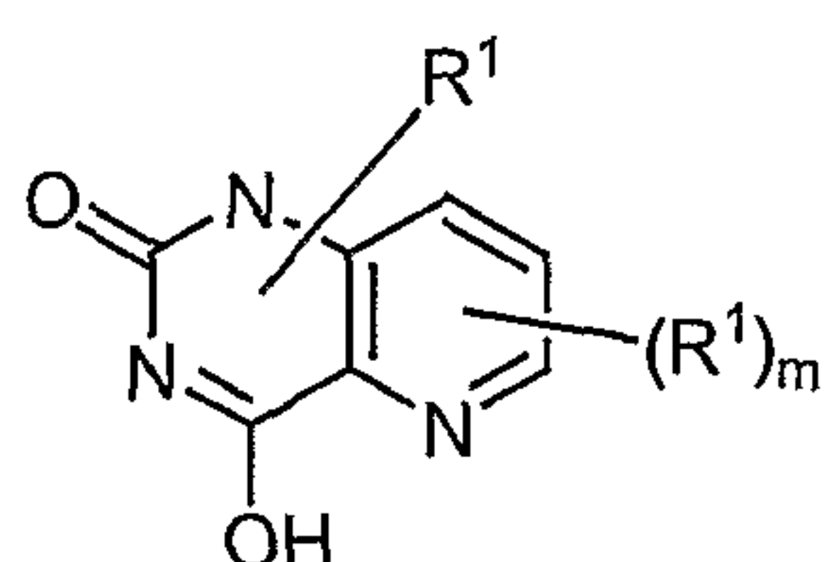
4-hydroxy-1H-pyrido[3,2-d]pyridin-2-one
