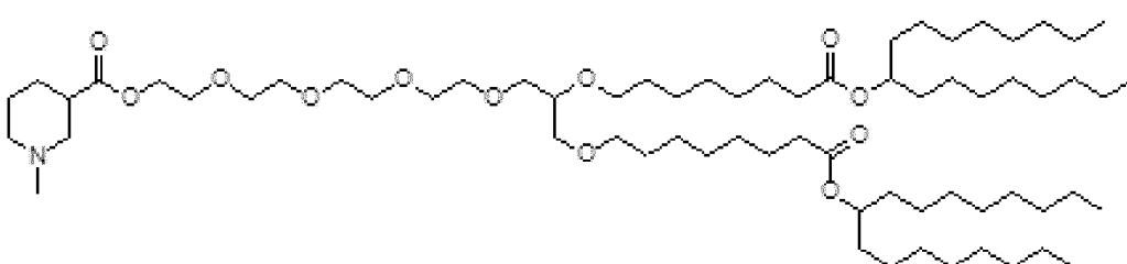
Compound XIX (Example 14)
