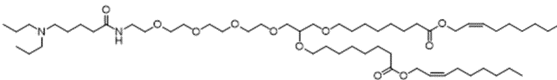
Compound XXVIII (Example 20)
