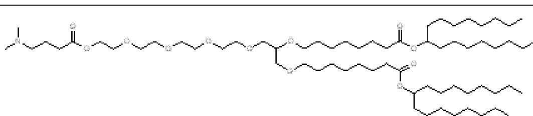
Compound XXII (Example 17)
