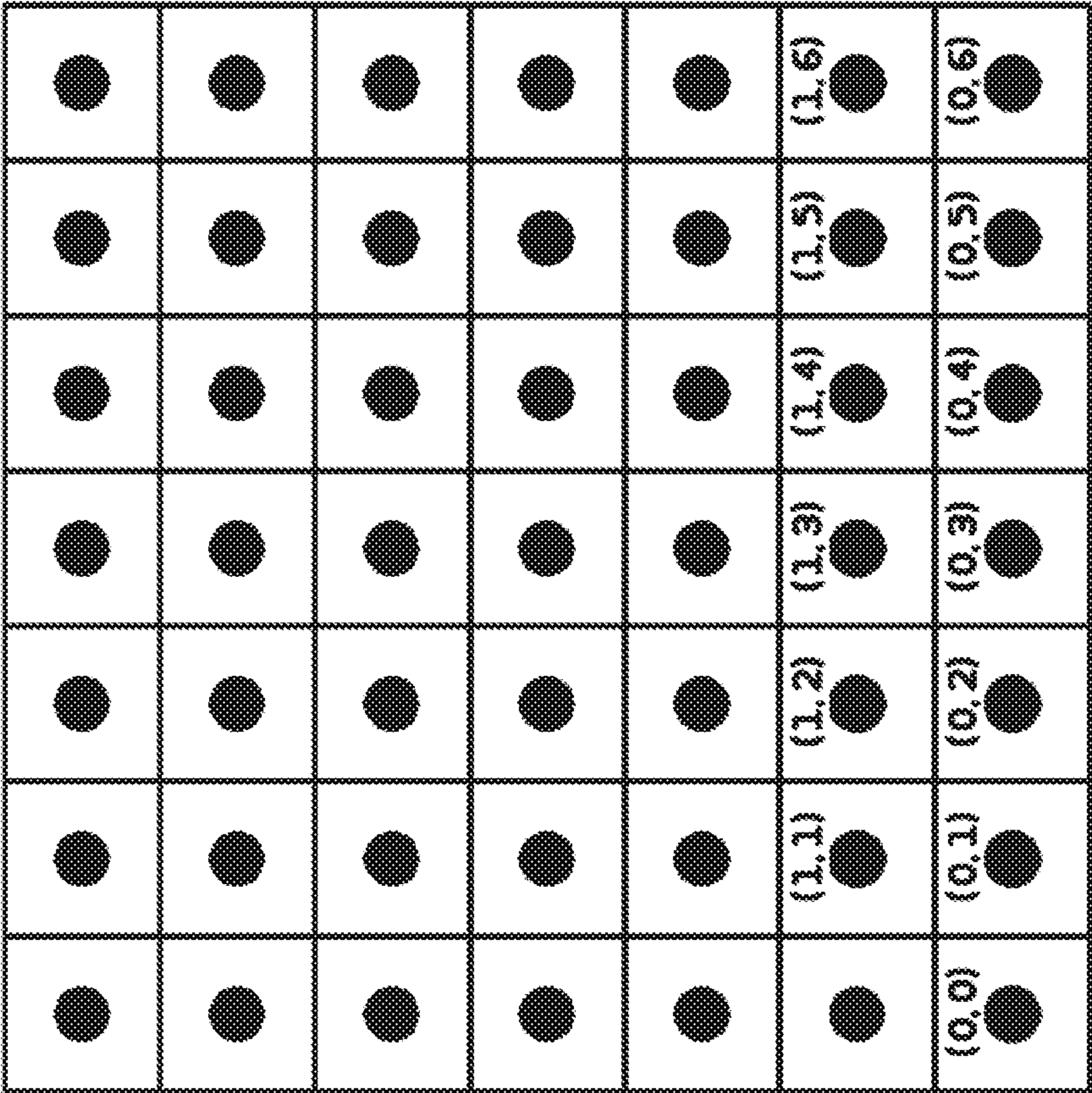
Coordinates (x,y) in cartesian space
