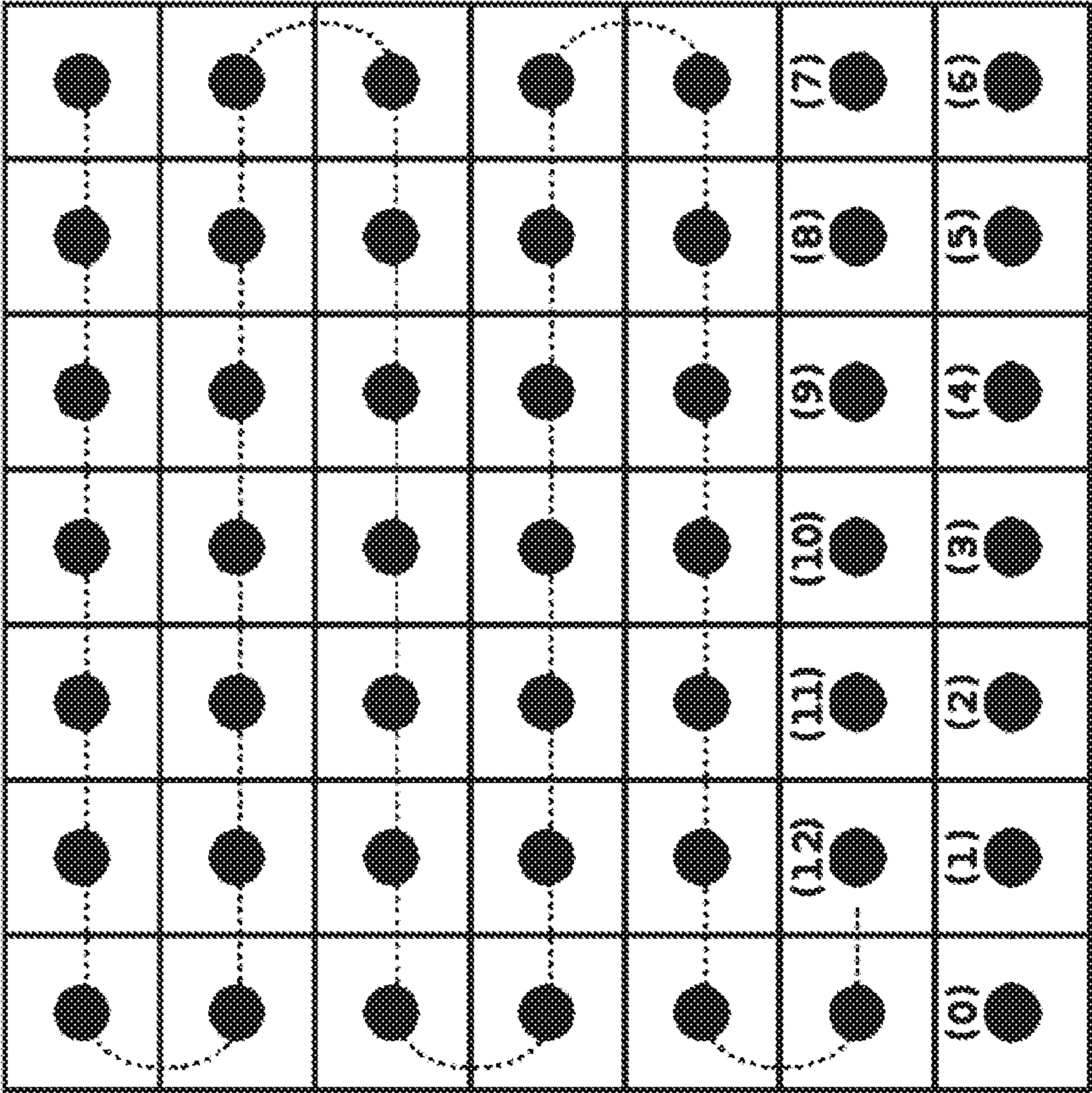
Parameter (t) of Nonlinear curve C(t)
