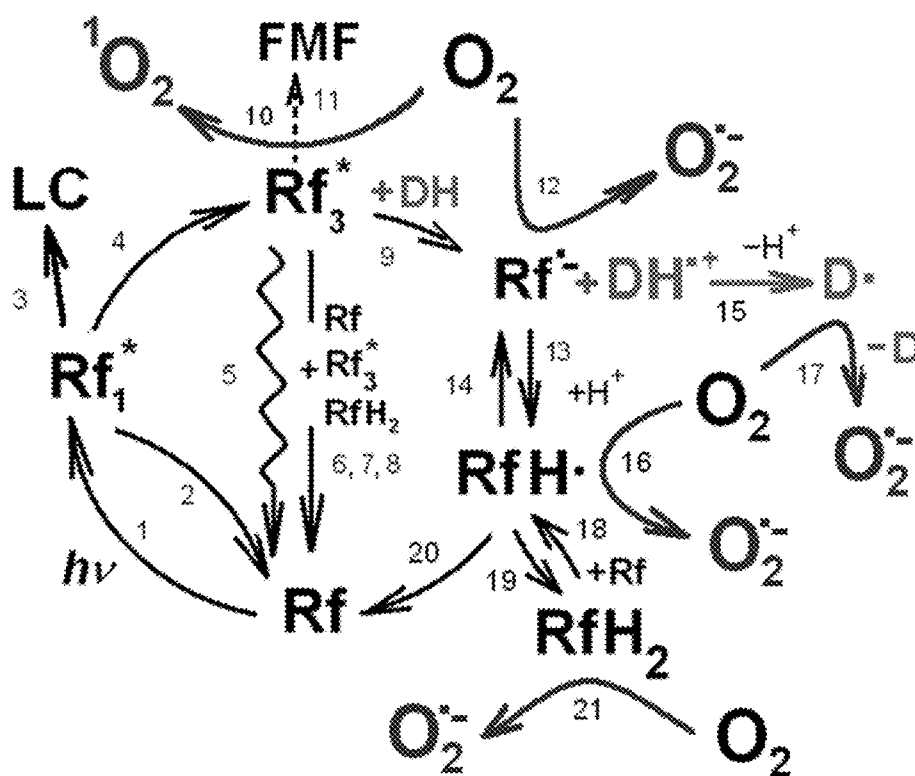
Scheme 1 – Simplified mechanism of photochemical transformations of riboflavin under light (lumichrome (LC), 1,5-dihydroflavin ( RfH_2 ), formylmethylflavin (FMF), superoxide anion ( O_2^{\bullet-} ), electron donor group (DH))
