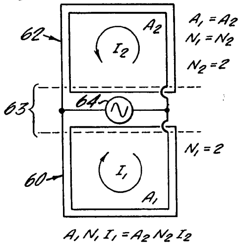
Fig. 5 (PRIOR ART)
