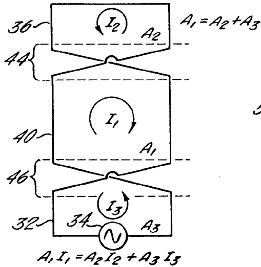
Fig. 5 (PRIOR ART)
