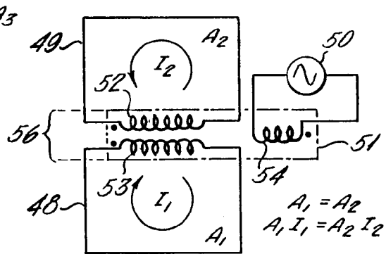
Fig. 6 (PRIOR ART)
