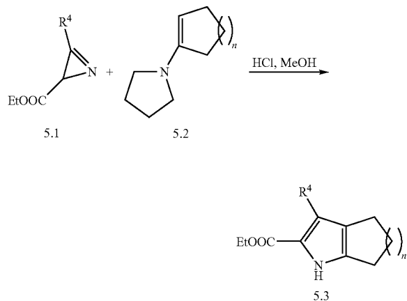
Scheme 5: Synthesis of Compounds including R 4
