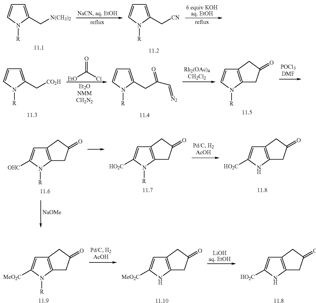
Scheme 11: Synthesis of a 5-Keto Analogs
