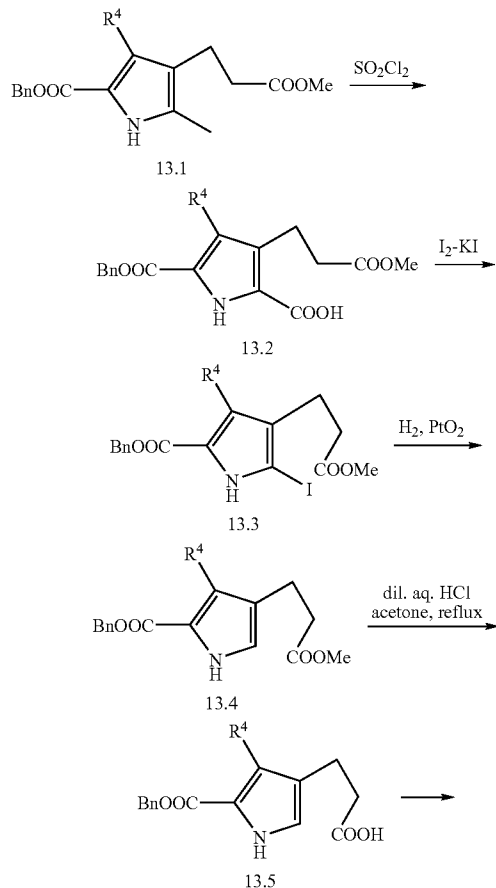
Scheme 13: Synthesis of 6-Keto Analogs (13.8)
