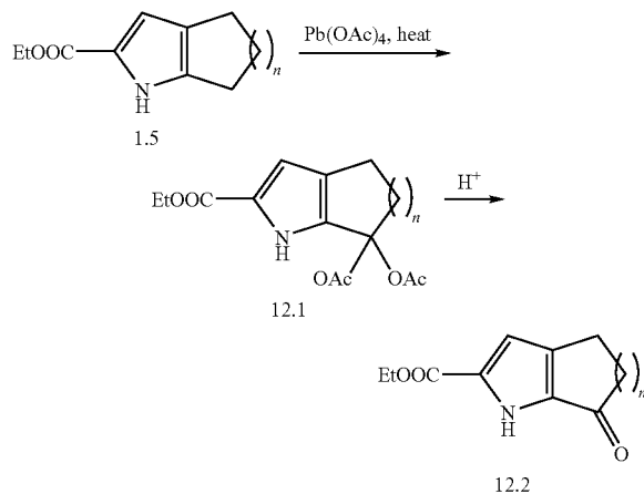
Scheme 12: Synthesis of 6-Keto Analogs (12.2)
