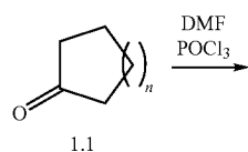
Scheme 3: Synthesis of Core Scaffold
