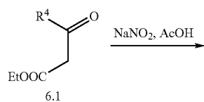
Scheme 9: Synthesis of 4-Keto Analogs (9.2)
