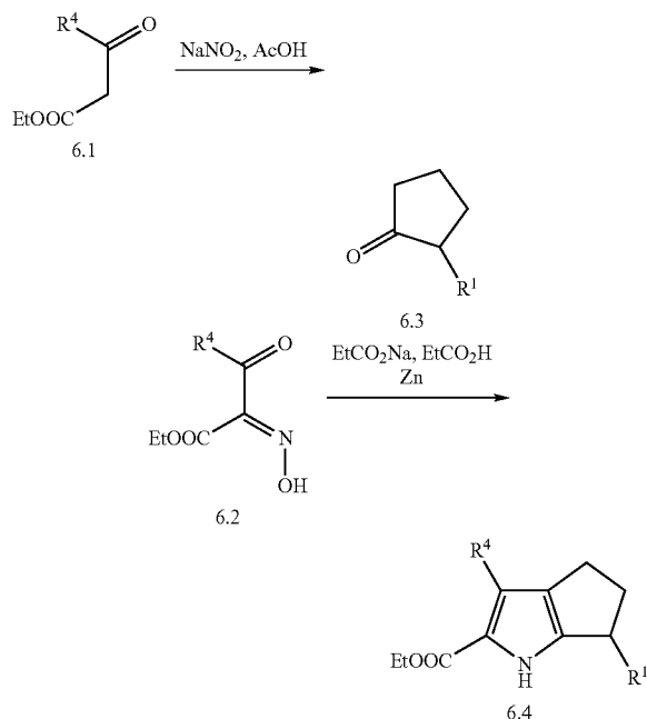
Scheme 6: Synthesis of Scaffold 6.4
