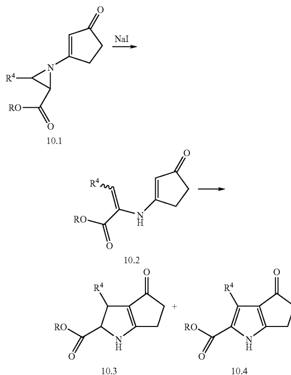
Scheme 10: Synthesis of 4-Keto Analogs (10.4)
