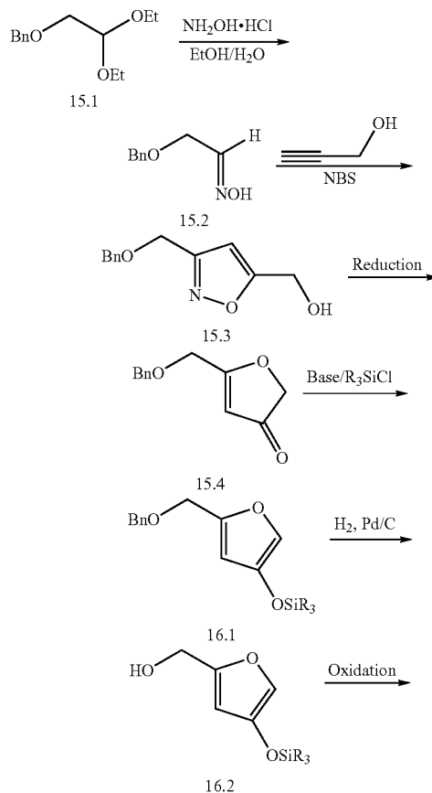
Scheme 16: Synthesis of Difluoro Analog (16.5)
