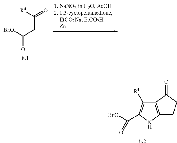
Scheme 8: Synthesis of 4-Keto Analogs (8.2)
