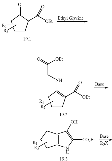
Scheme 19: Synthesis of hydroxy (18.3) and alkoxy-substituted analogs (19.4)
