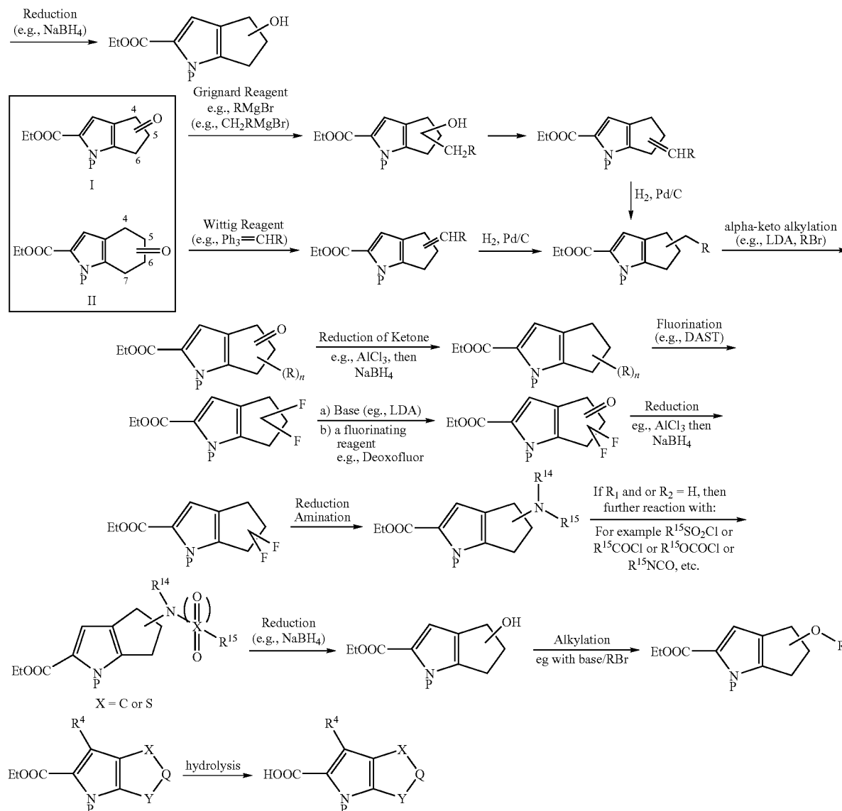
Scheme 14: Synthesis of Substituted Analogs from Keto Intermediates
