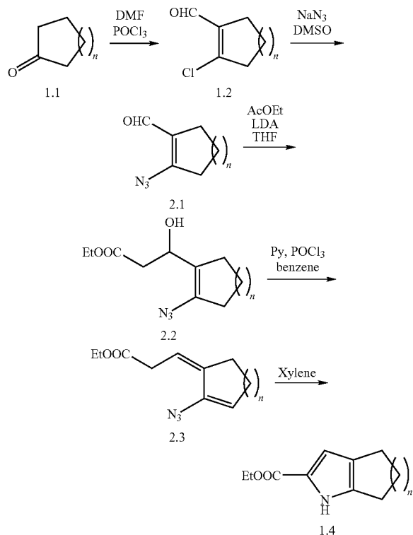
Scheme 2: Synthesis of Core Scaffold
