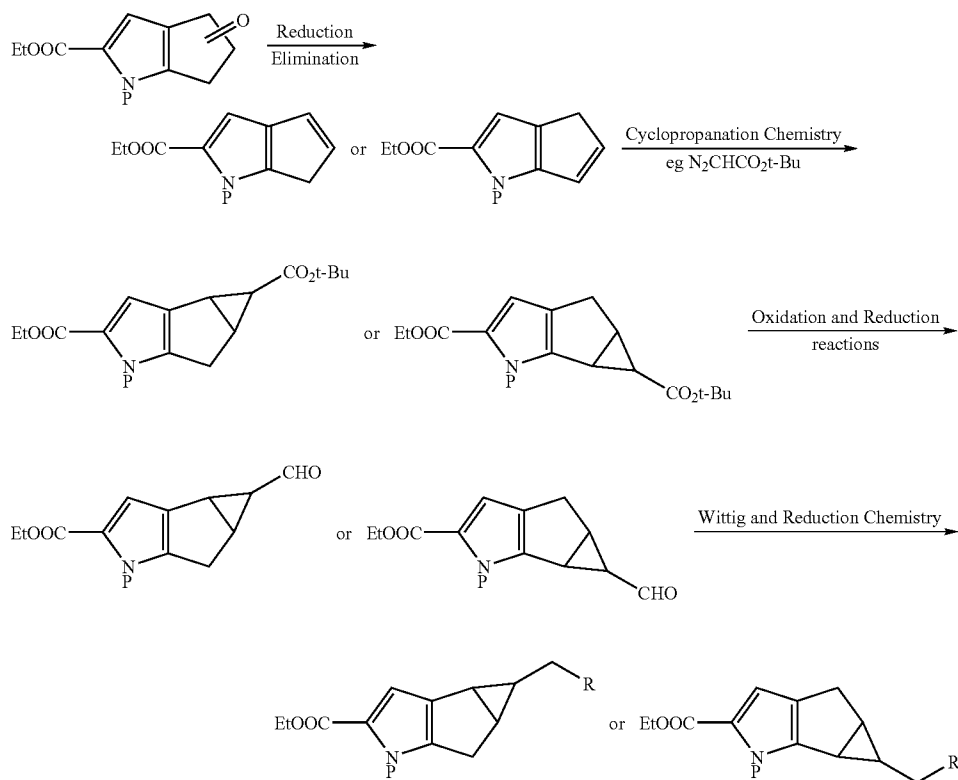
Scheme 18: Synthesis of Cyclopentadiene and Cyclopentane Intermediates
