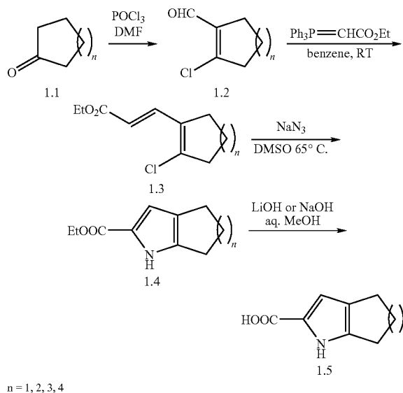
Scheme 1: Synthesis of Core Scaffold
