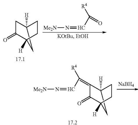
Scheme 17: Synthesis of Bridged Analogs (17.7)
