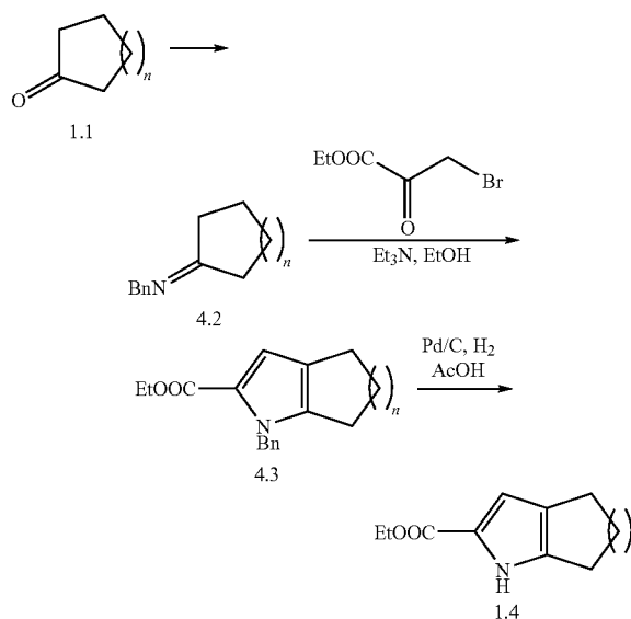
Scheme 4: Synthesis of Core Scaffold
