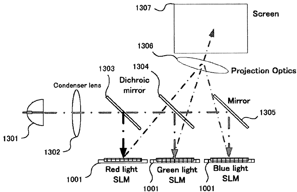
Projection display system of 3 SLMs
