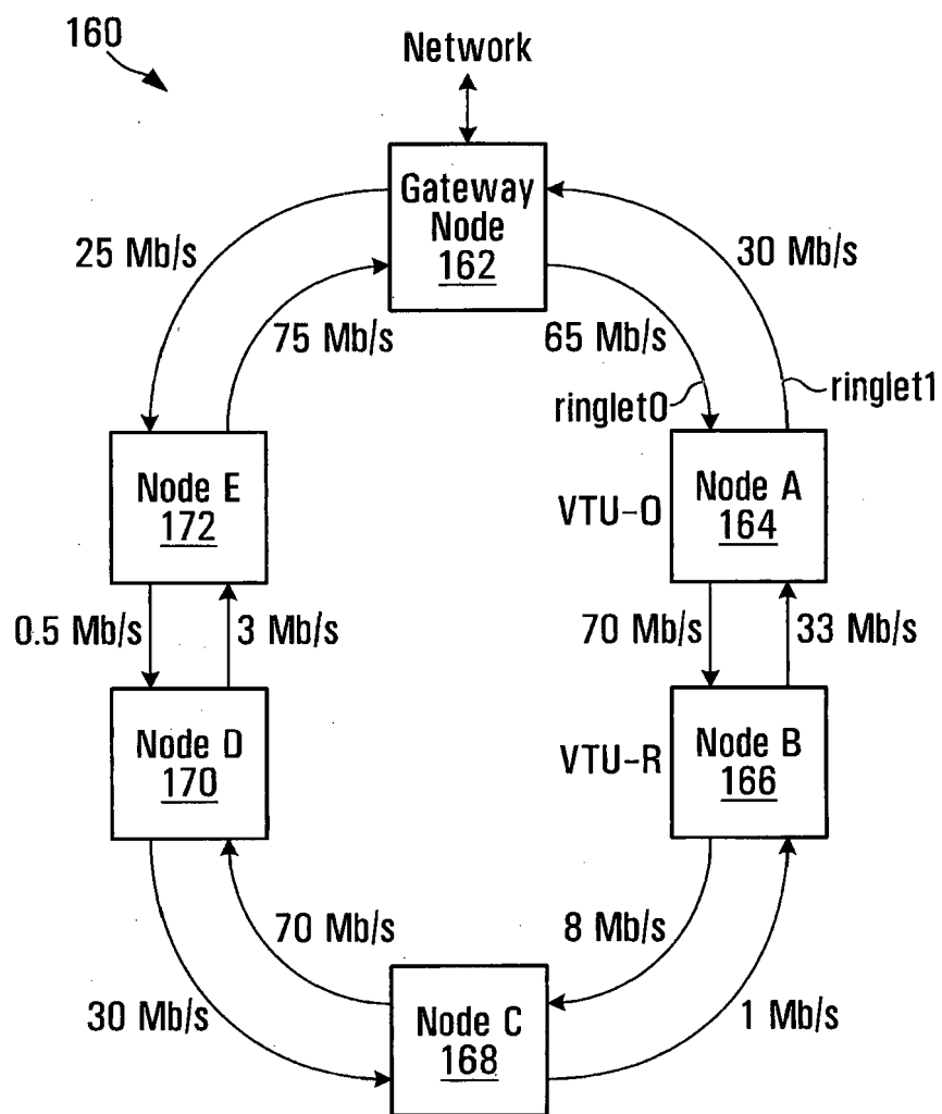
Ring with Inherent Bandwidth Bottlenecks
