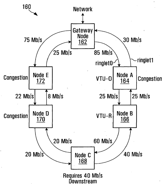
Asymmetric DSL Rings Dynamically Optimized Ring
