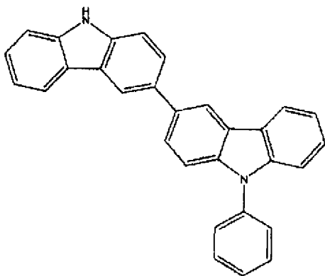
Intermediate body 1-4
