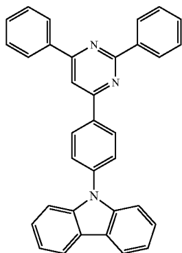
Compound D
