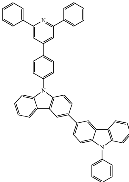
Compound 2
