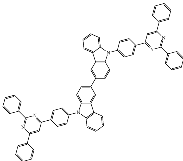
Compound 4
