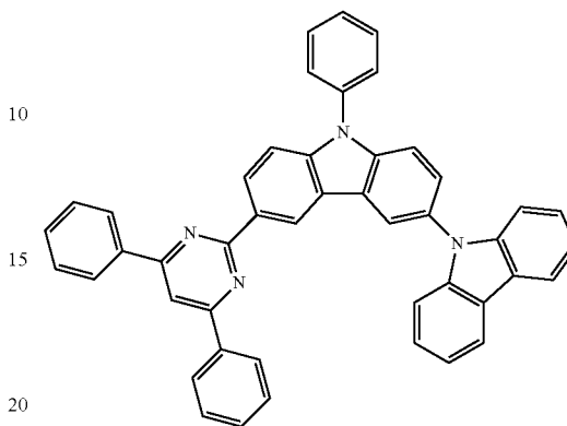
Compound G
