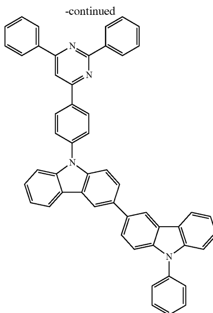
Compound 1
