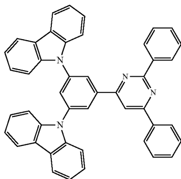
Compound E
