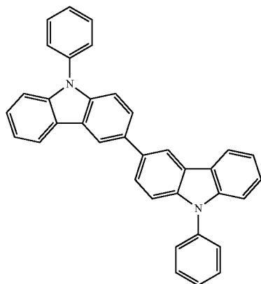
Compound F
