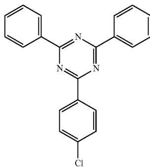
Intermediate body 3-2
