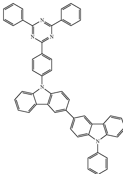
Compound 3
