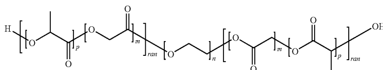
triblock-type polymer
