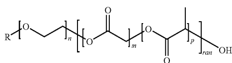
diblock-type polymer
