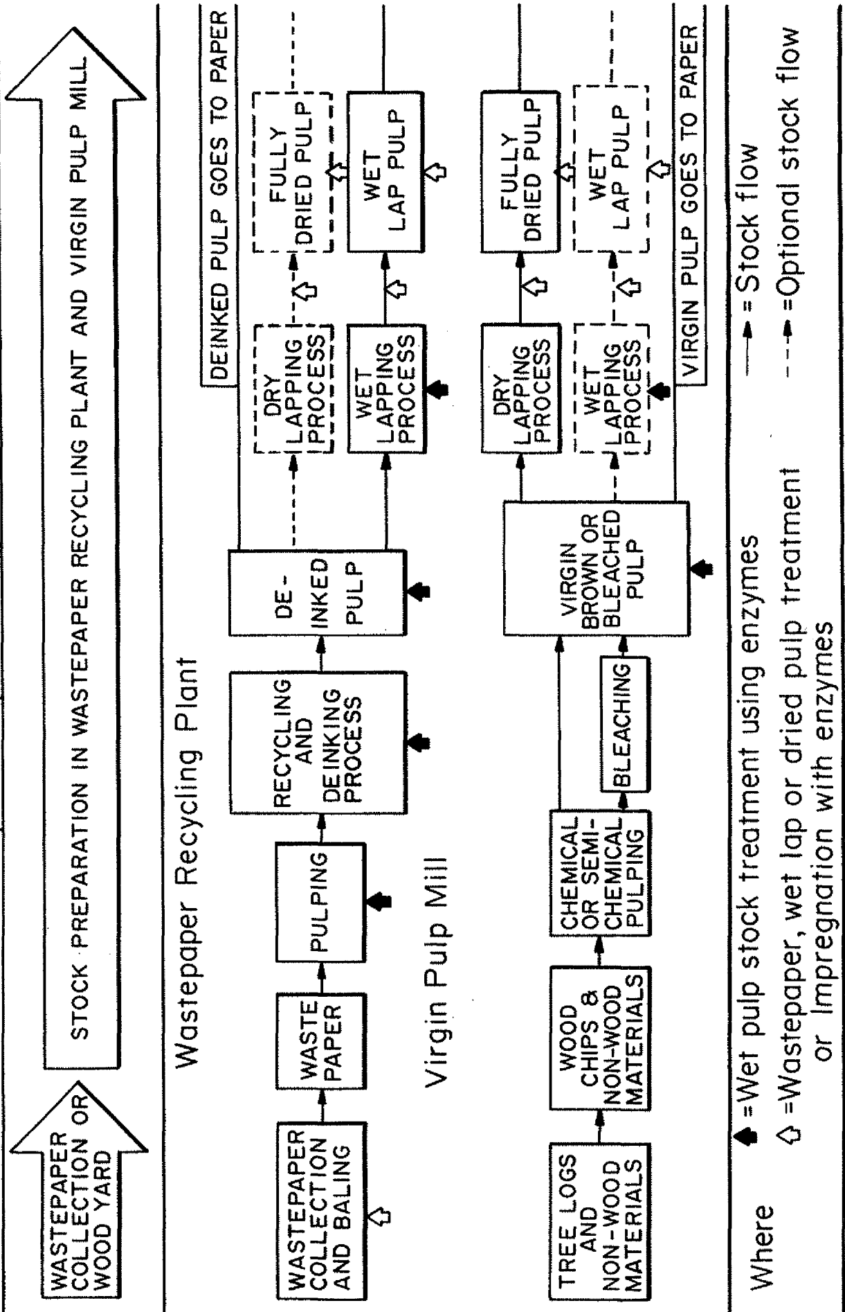
FIG. 1 Pulp and Paper Making Processes Schematic
