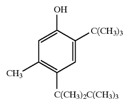
2-tert-butyl-4-(1,1,2,2-tetramethylpropyl)-5-methylphenol and
