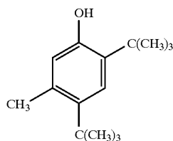
2,4-di-t-butyl-5-methylphenol
