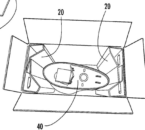
FIG. 1C (PRIOR ART)
