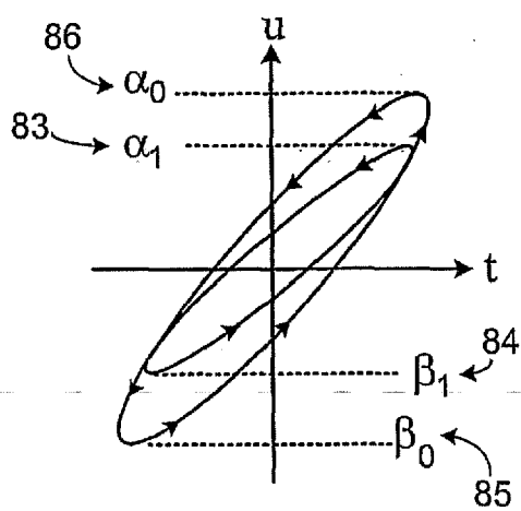
MINOR HYSTERESIS LOOP
