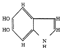
5,6-dihydroxyindole (DHI)
