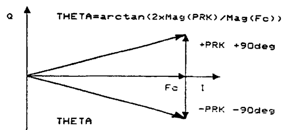
Figure 4(a) : Phasor diagram showing Excitation and Modulation
