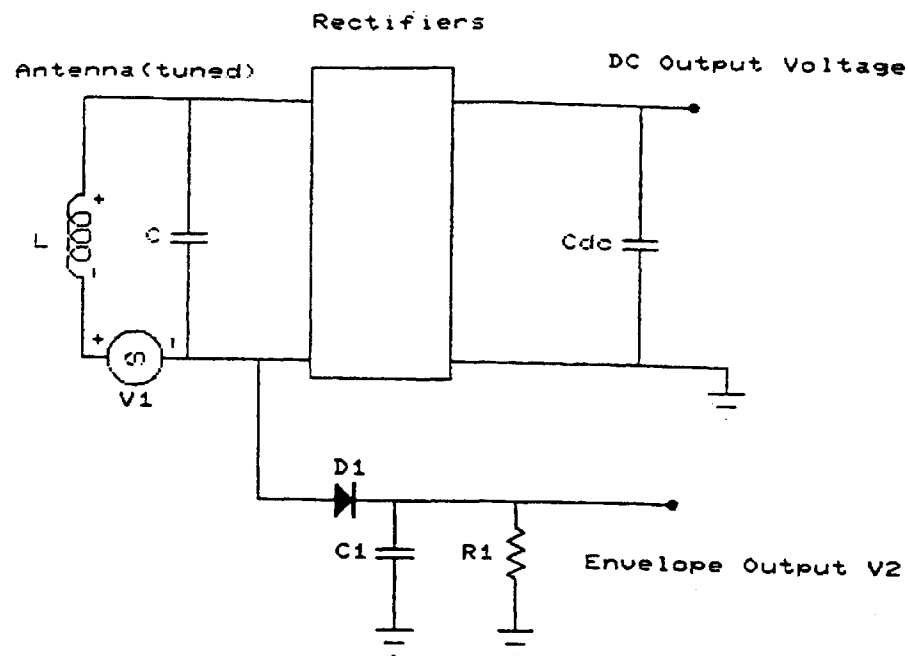
Figure 1 : Prior Art Transponder
