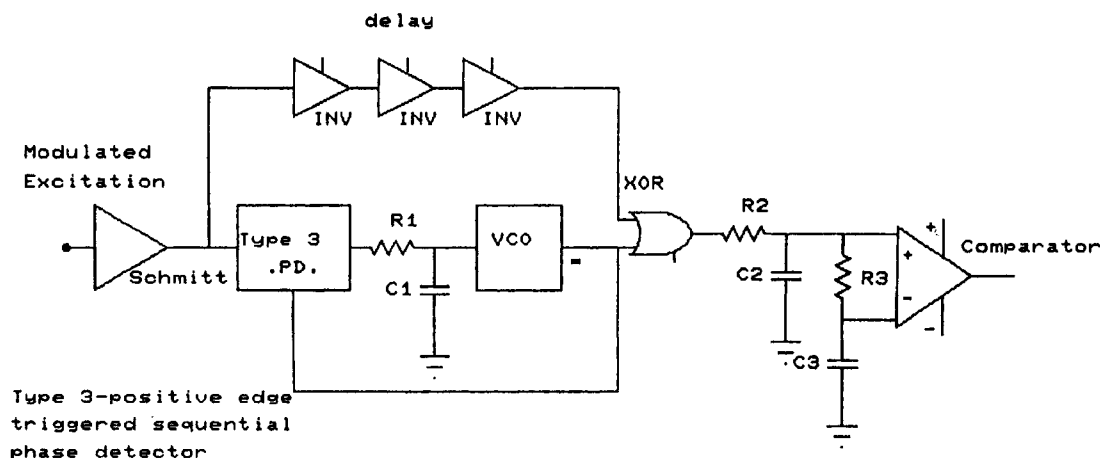
Example Circuit for Demodulating
