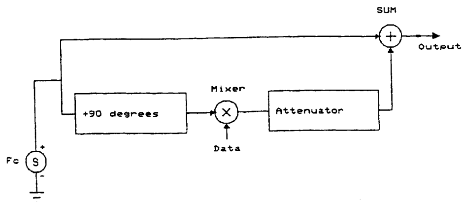
Figure 6(a) : Method of Modulating Excitation Signal
