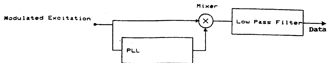
Figure 6(b) : Method of Demodulation
