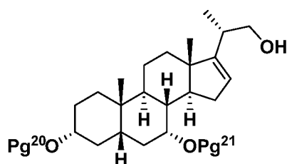
Formula IV-2
