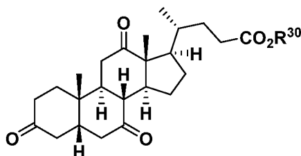
Formula III-6;
