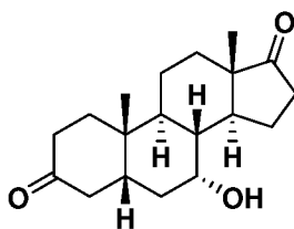
Formula III-11;
