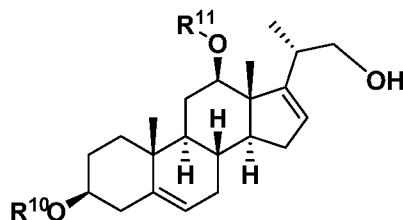
Formula II-1
