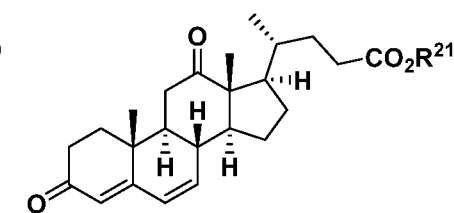
Formula II-6
