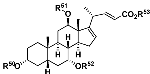
Formula V-3
