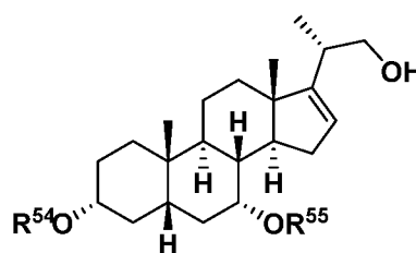
Formula V-6
