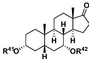
Formula IV-6
