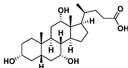
Compound 33
