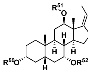
Formula V-4
