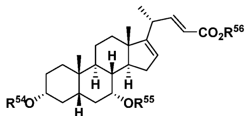
Formula V-8;
