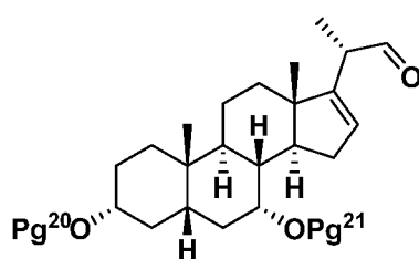
Formula IV-3;
