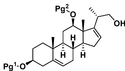
Formula I-11
