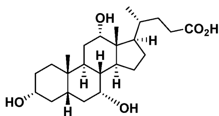
Cholic acid
