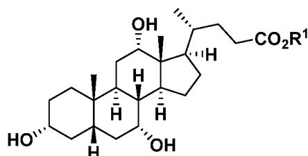
Formula I-6
