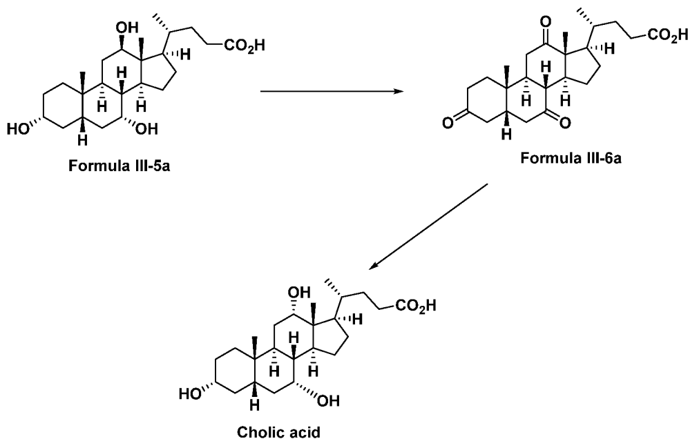
Scheme 5a
