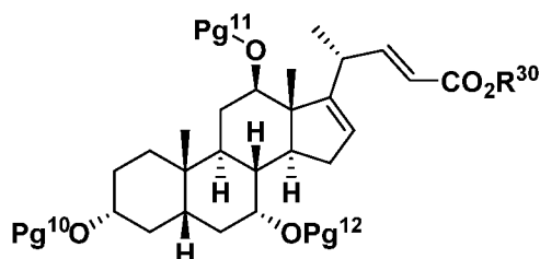
Formula III-4;
