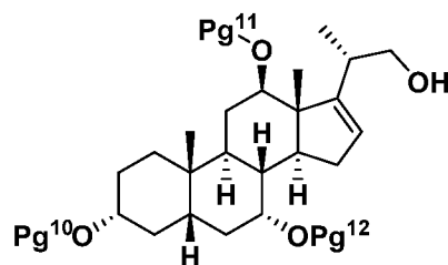
Formula III-2
