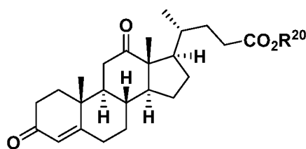
Formula II-5
