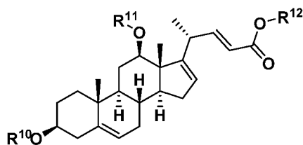
Formula II-3
