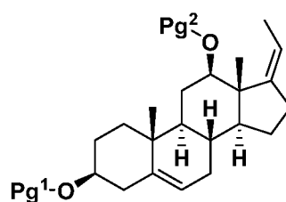
Formula I-10
