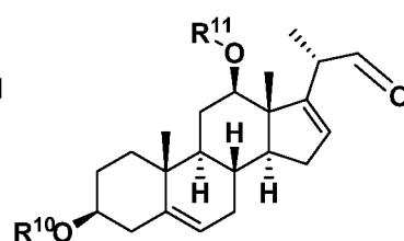
Formula II-2
