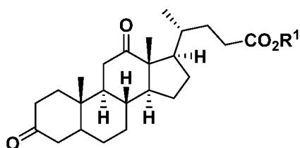
Formula I-1
