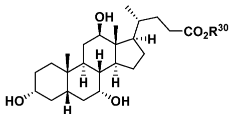
Formula III-5;
