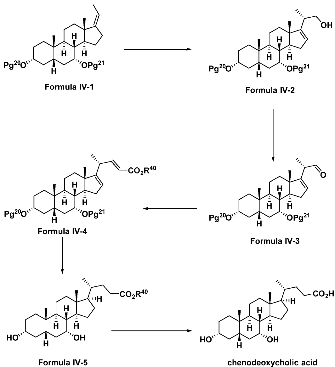
Scheme 8
