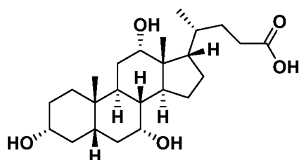
Compound 34
