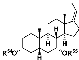
Formula V-5
