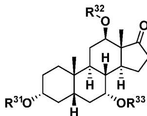
Formula III-8
