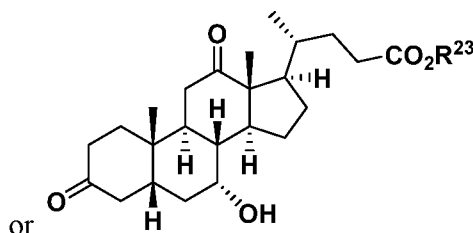
Formula II-8
