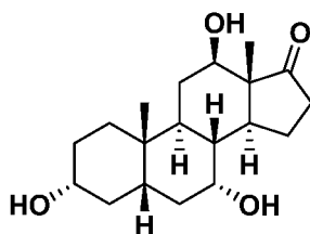
Formula III-8a;
