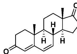
Formula III-9;
