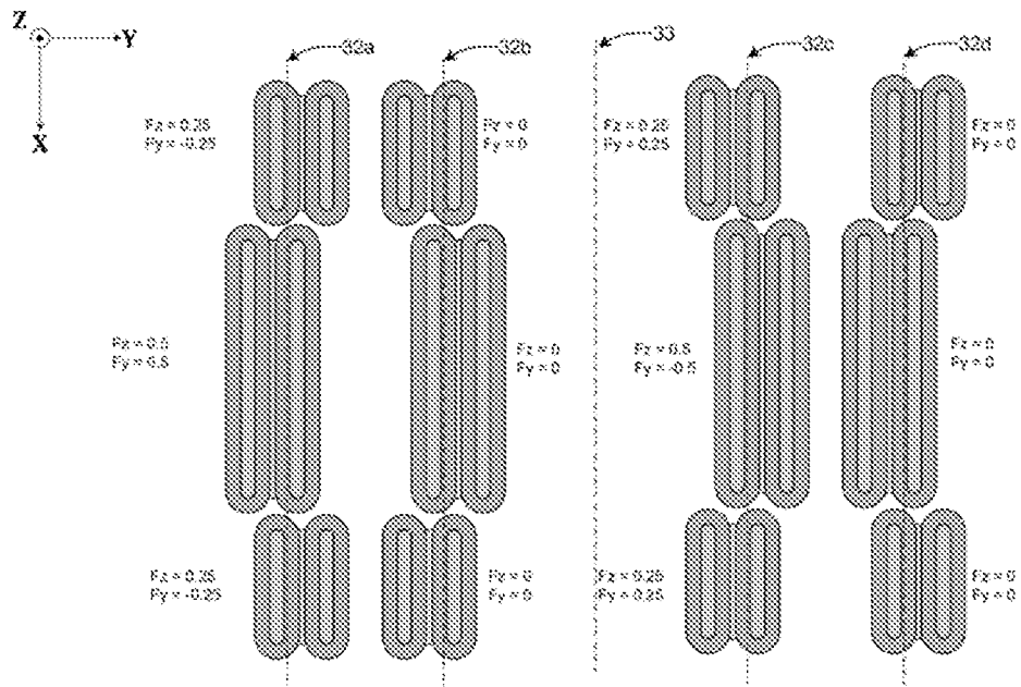
Controllable Driving Method for Constant net F_z Net F_y Requirement Distributed on Two Guideways Only Net F_x Requirement Distributed on Two Guideways Only
