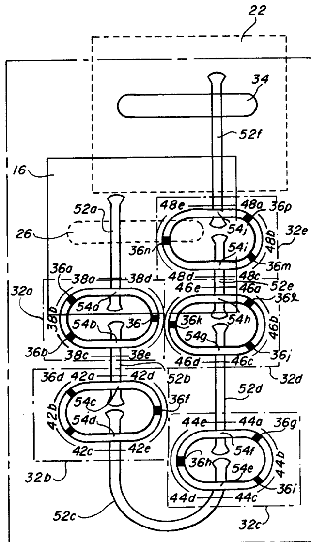
STRIPLINE-TO-SLOTLINE DIGITAL PHASE SHIFTER
