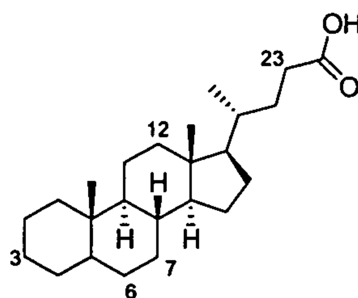
cholanic acid
